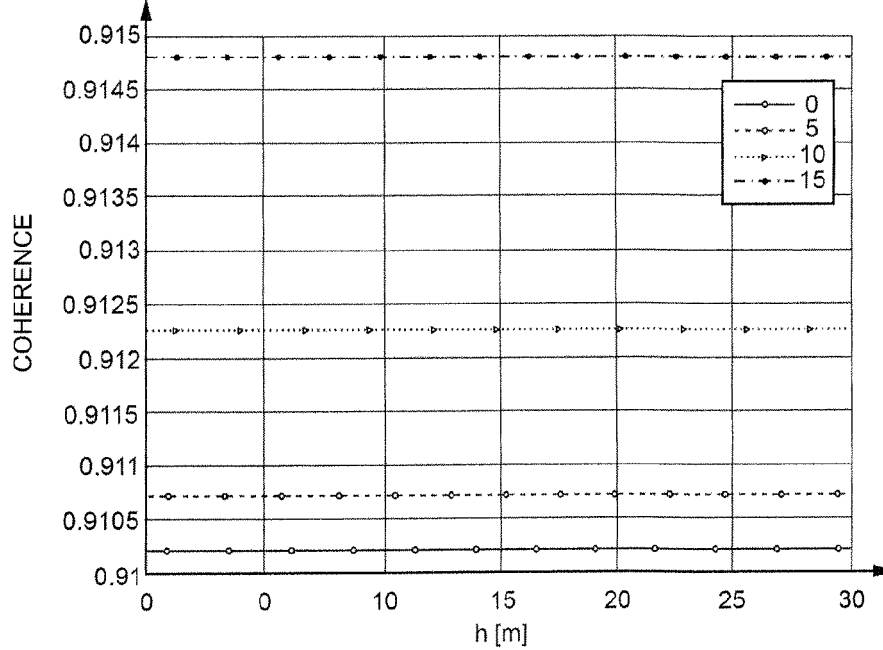
COHERENCE AS A FUNCTION OF TARGET HEIGHT AND MEAN SQUINT ANGLE BASELINE = 2 Km - ROLL ANGLE = 30° - SATELLITE HEIGHT = 619 Km
