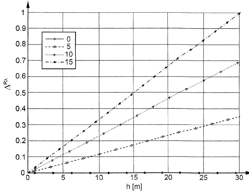
NORMALIZED DIFFERENCE OF PATH AS A FUNCTION OF TARGET HEIGHT AND MEAN SQUINT ANGLE BASELINE = 2 Km - ROLL ANGLE = 30° - SATELLITE HEIGHT = 619 Km
