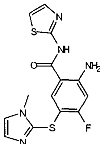
Banyu/Merck glucokinase activator
