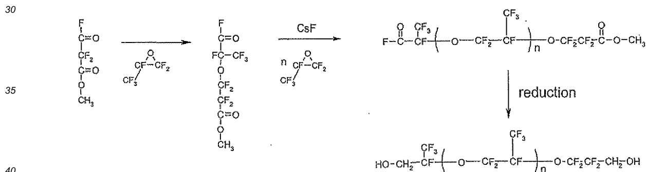
Scheme 3. Synthesis of a liquid PFPE precursor material from hexafluoropropylene oxide or tetrafluoro ethylene oxide.
