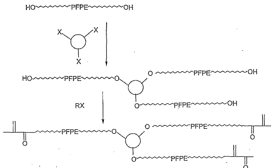
Scheme 4. Linker group joining three PFPE chains.
