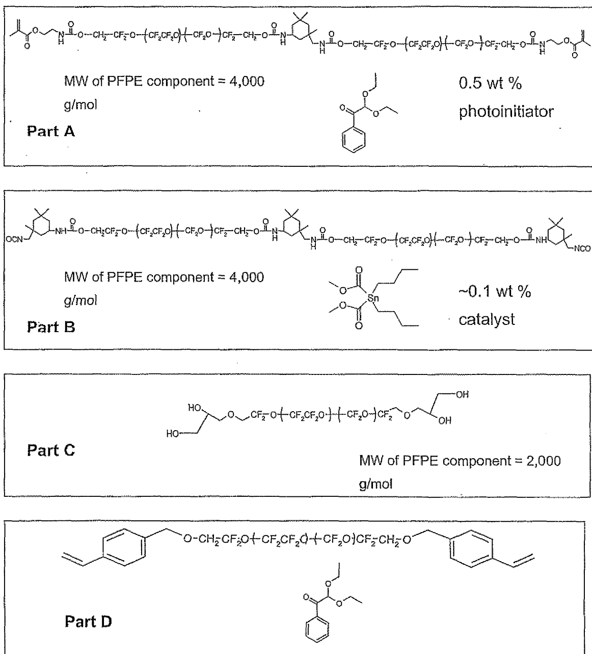
Scheme 7. PFPE Urethane System for Microfluidics.
