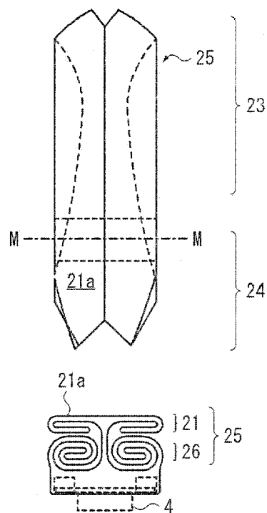
M-M SECTIONAL VIEW
