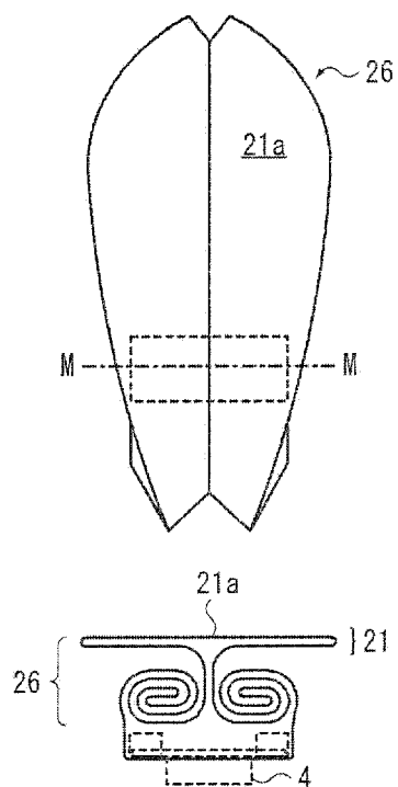
M-M SECTIONAL VIEW
