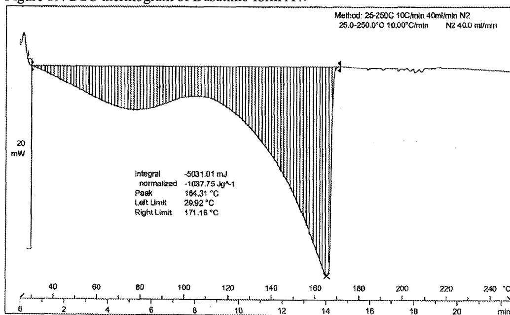
Figure 89: DSC thermogram of Dasatinib form AW
