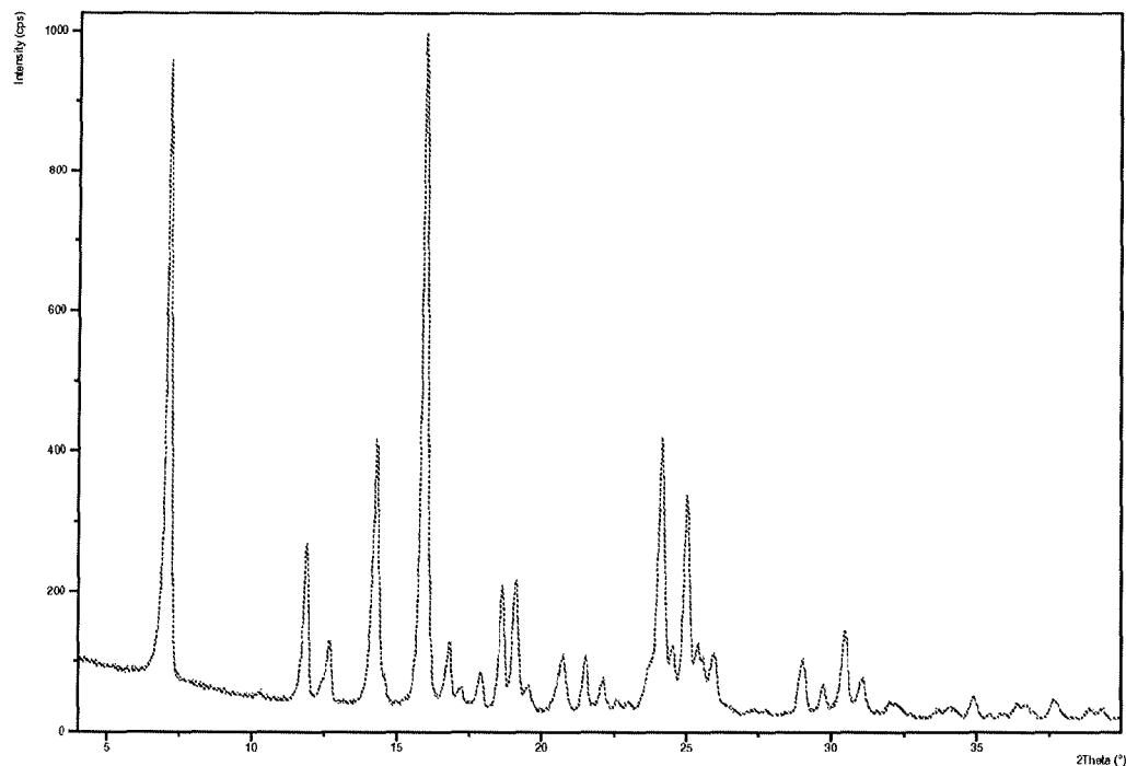
Figure 107: PXRD pattern of wet Dasatinib form AJ
