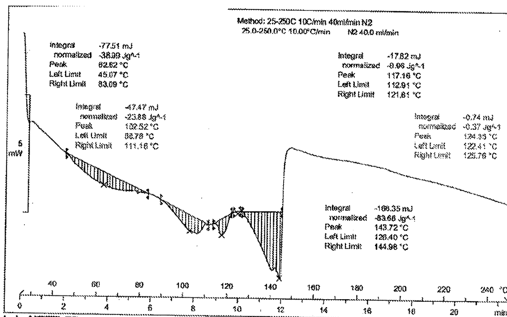
Figure 67: DSC thermogram of Dasatinib form AK
