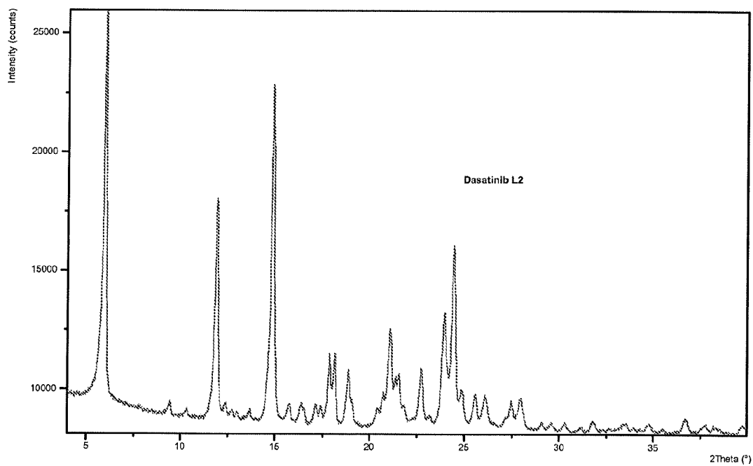
Figure 12: PXRD pattern of Dasatinib form L2
