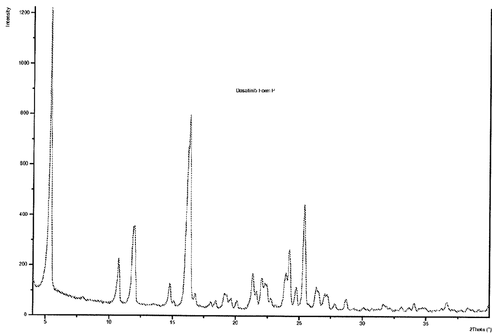
Figure 24: PXRD pattern of Dasatinib form P
