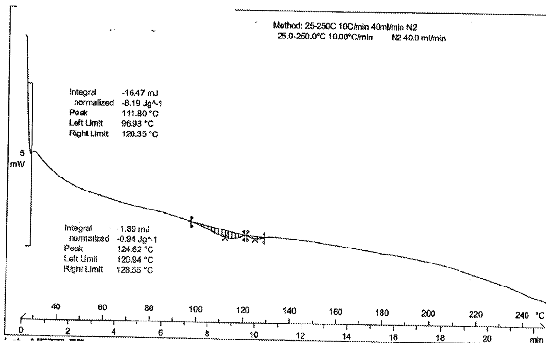
Figure 71: DSC thermogram of Dasatinib form AM
