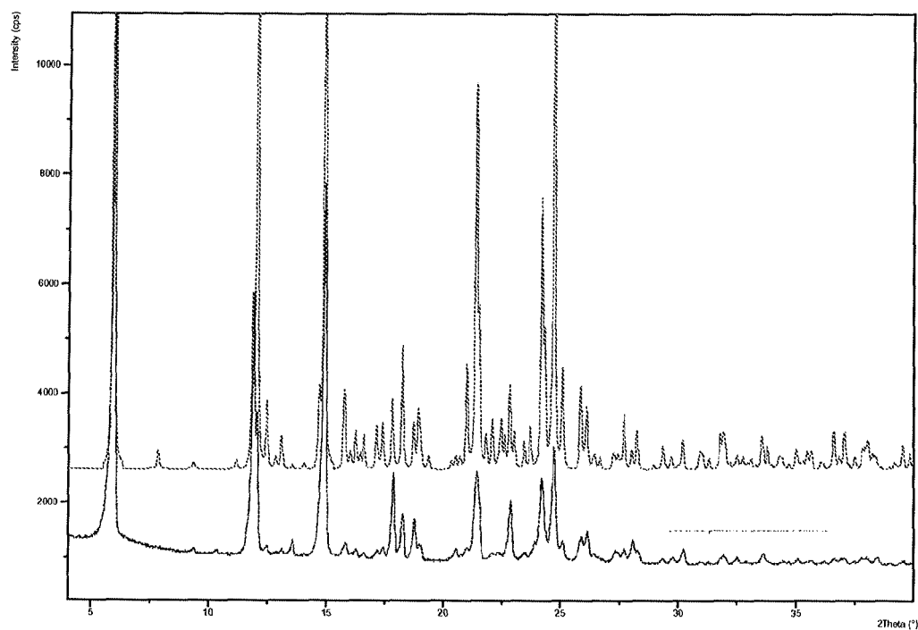
Figure 97: PXRD pattern of Dasatinib form BA
