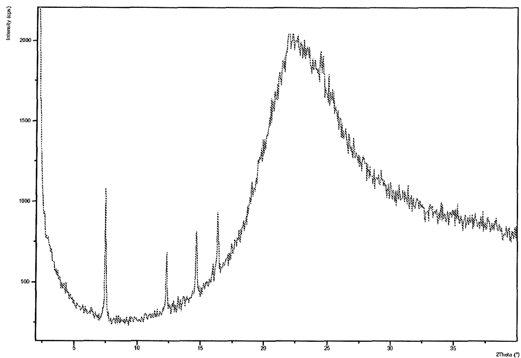
Figure 48: PXRD pattern of Dasatinib form AW
