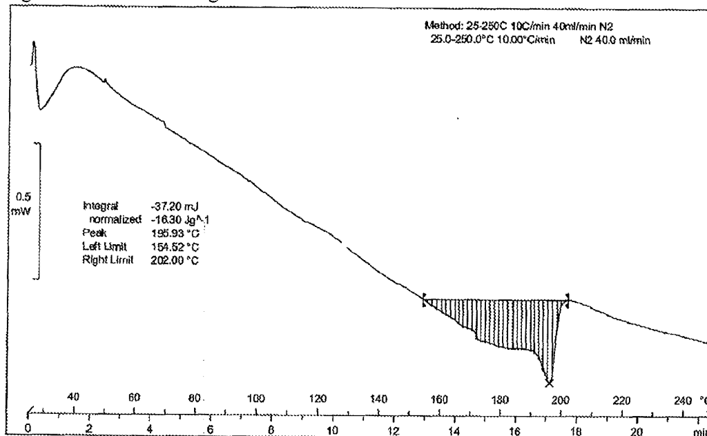
Figure 113: DSC thermogram of Dasatinib form BD
