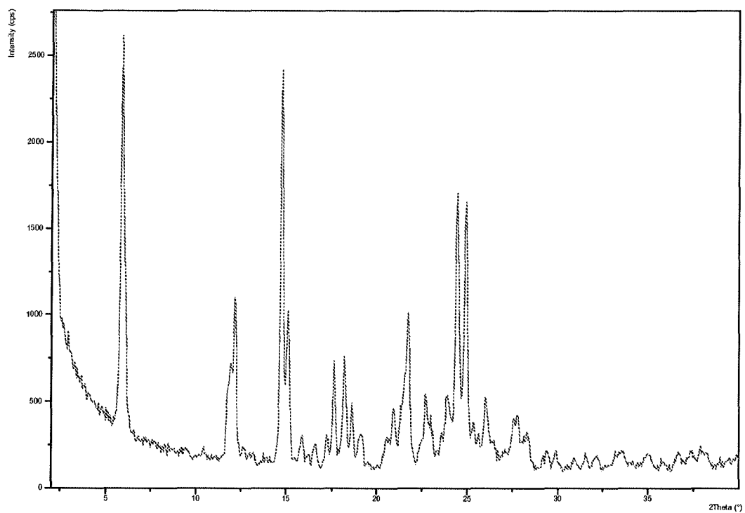
Figure 41: PXRD pattern of Dasatinib form AR
