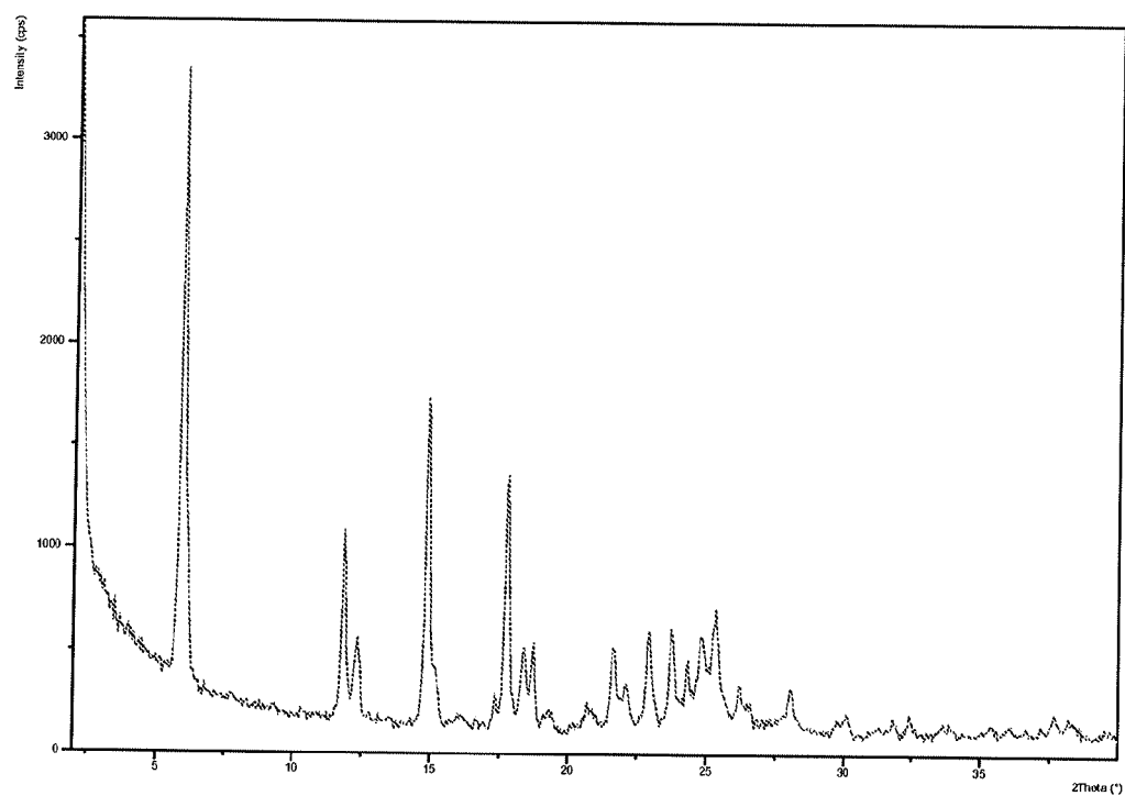
Figure 108: PXRD pattern of wet Dasatinib form AL
