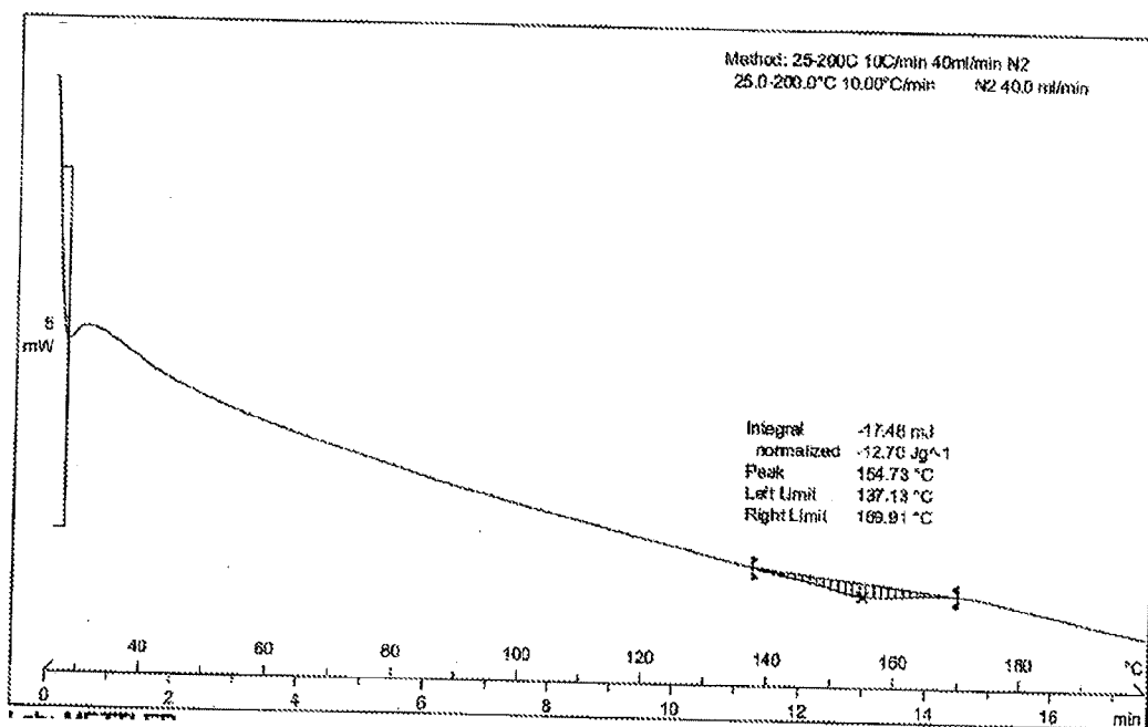
Figure 63: DSC thermogram of Dasatinib form AI
