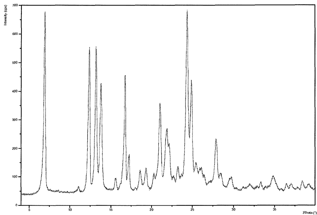
Figure 130: A powder XRD pattern of Dasatinib form N-6 (anhydrous)
