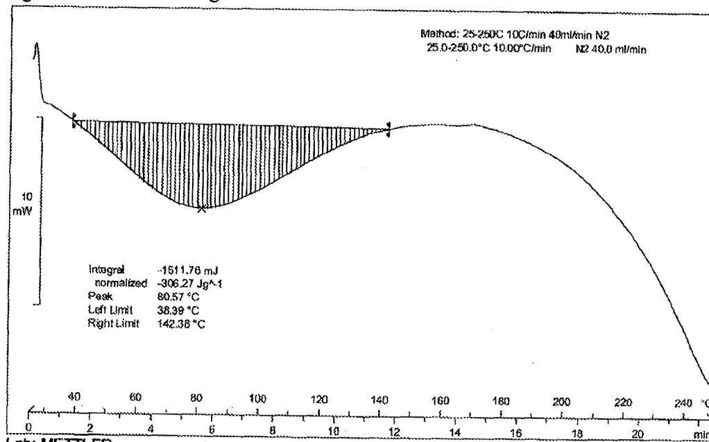
Figure 105: DSC thermogram of Dasatinib form BC
