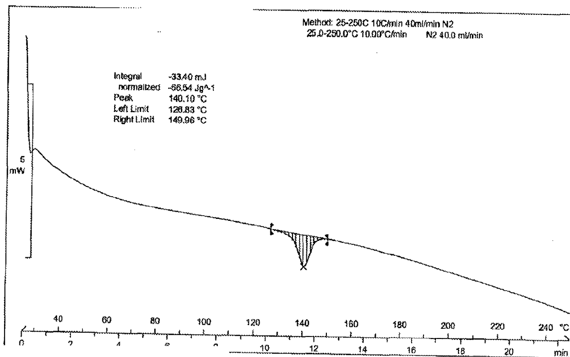
Figure 54: DSC thermogram of Dasatinib form AC
