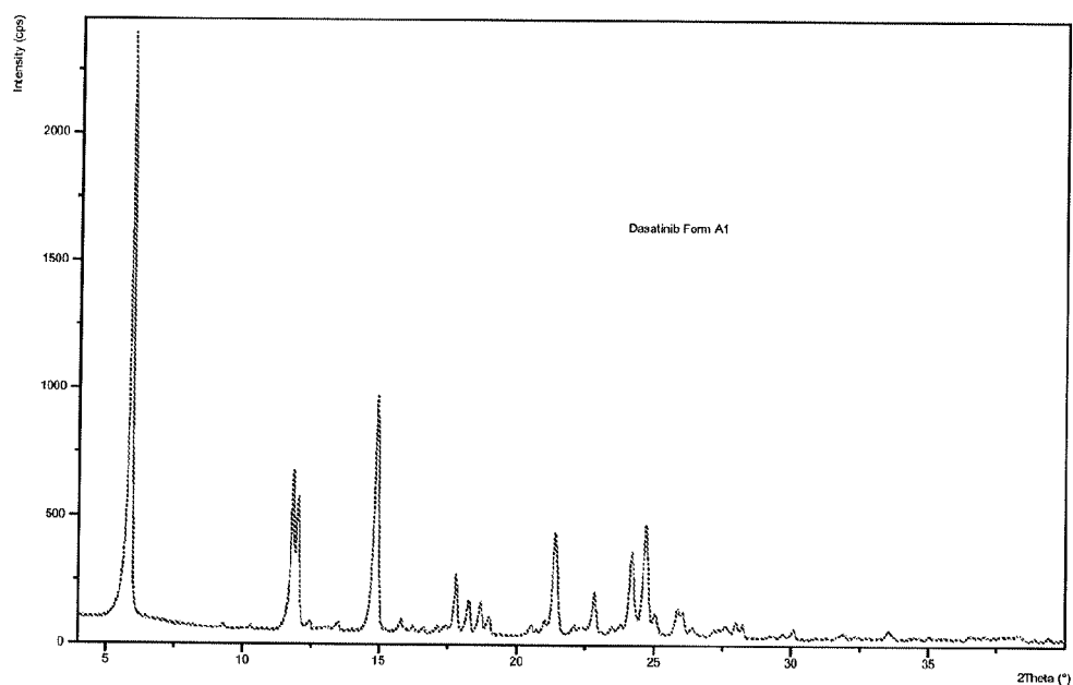
Figure 17: PXRD pattern of Dasatinib form A1
