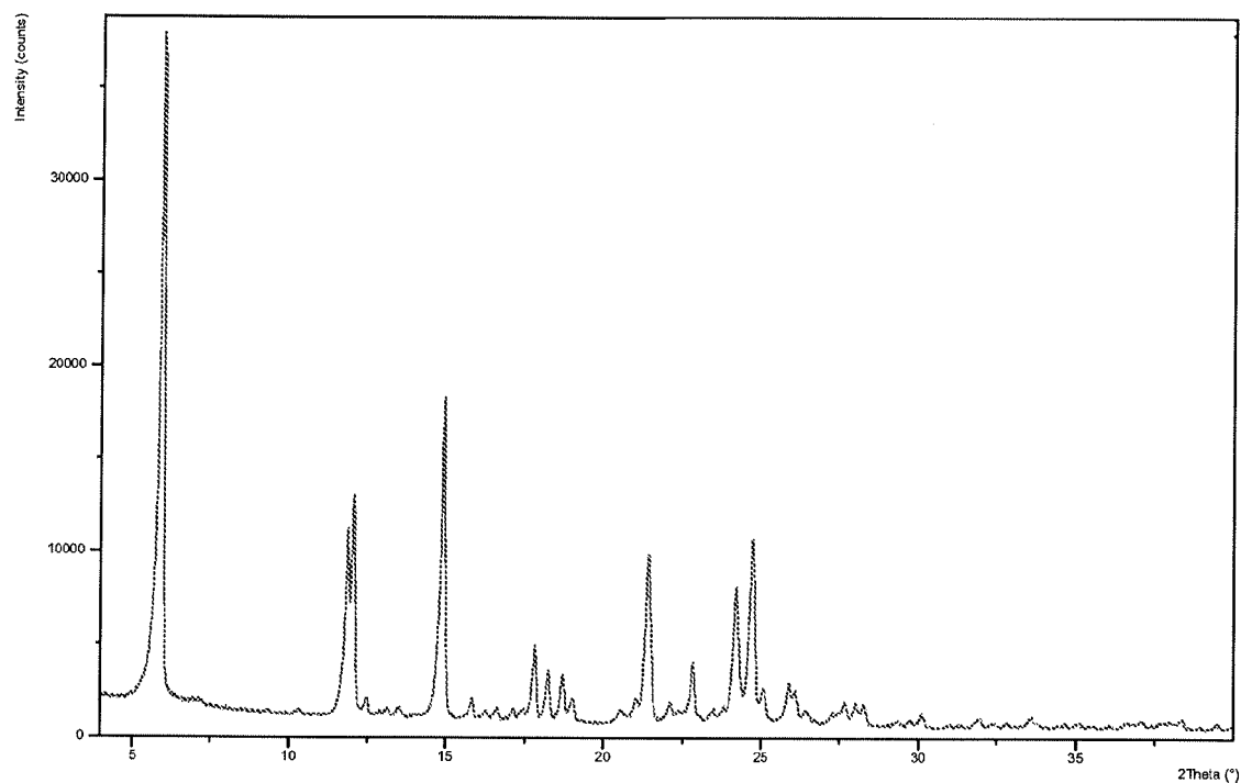
Figure 2: PXRD pattern of Dasatinib form B
