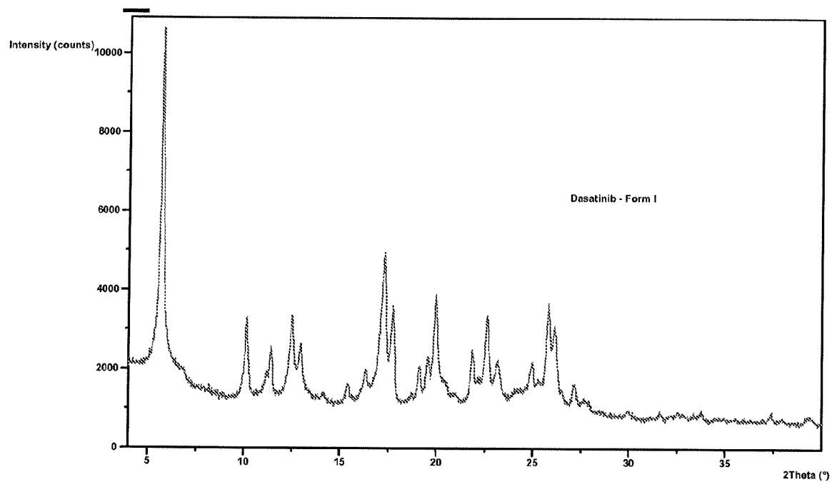
Figure 9: PXRD pattern of Dasatinib form I
