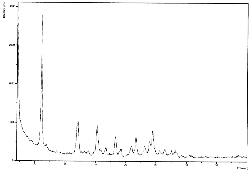
Figure 39: PXRD pattern of Dasatinib form AP
