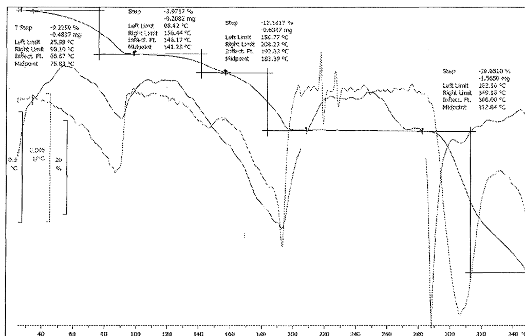
Figure 126: TGA thermogram of Dasatinib form BL
