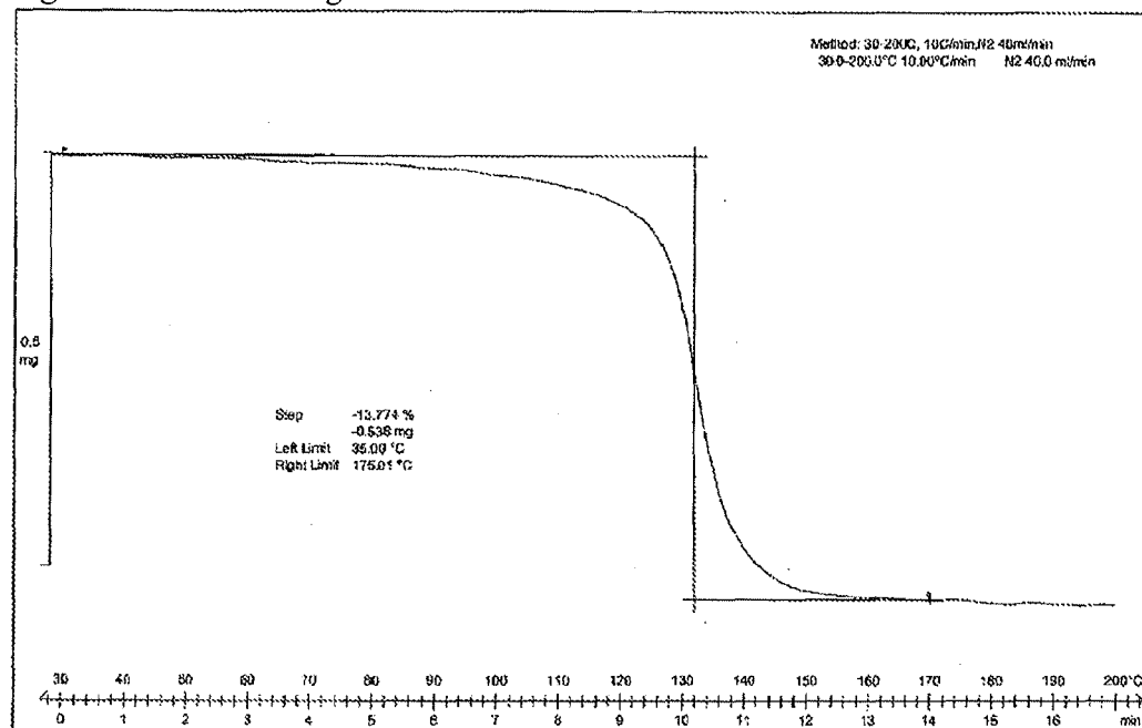
Figure 80: TGA thermogram of Dasatinib form AS
