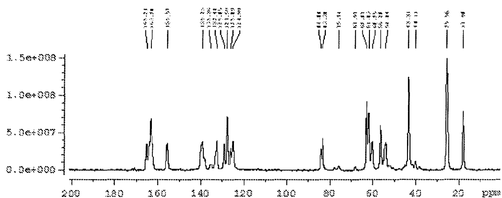
Figure 122: A detailed solid state ^{13}\text{C} NMR spectrum of dasatinib form A3.
