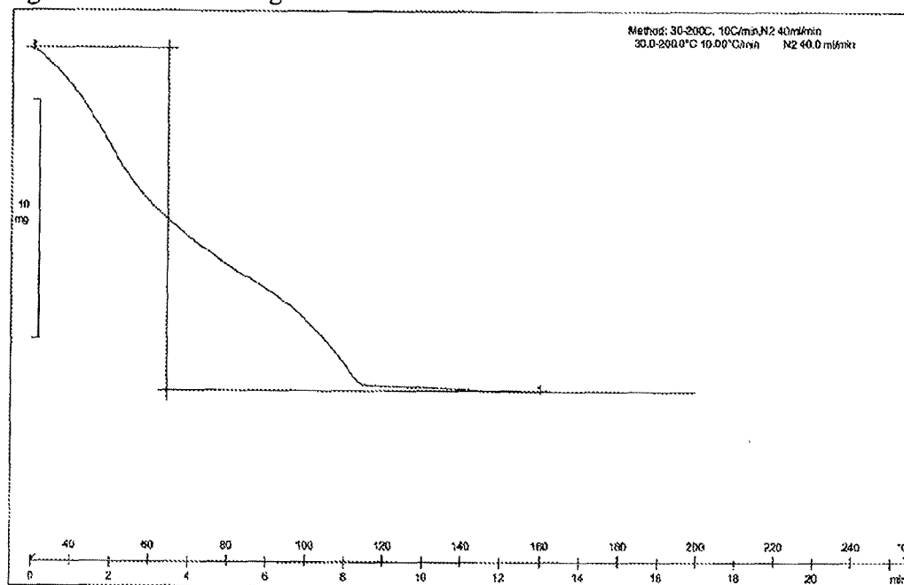
Figure 116: TGA thermogram of Dasatinib form BJ
