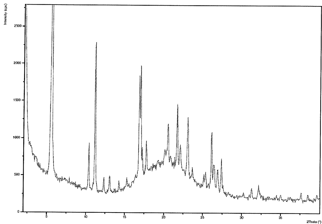
Figure 47: PXRD pattern of Dasatinib form AY
