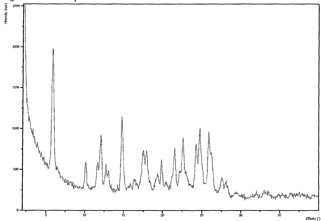
Figure 110: PXRD pattern of Dasatinib form BG
