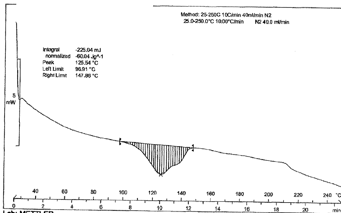
Figure 50: DSC thermogram of Dasatinib form AA
