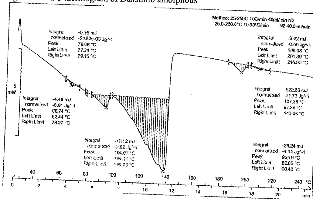
Figure 93: DSC thermogram of Dasatinib amorphous
