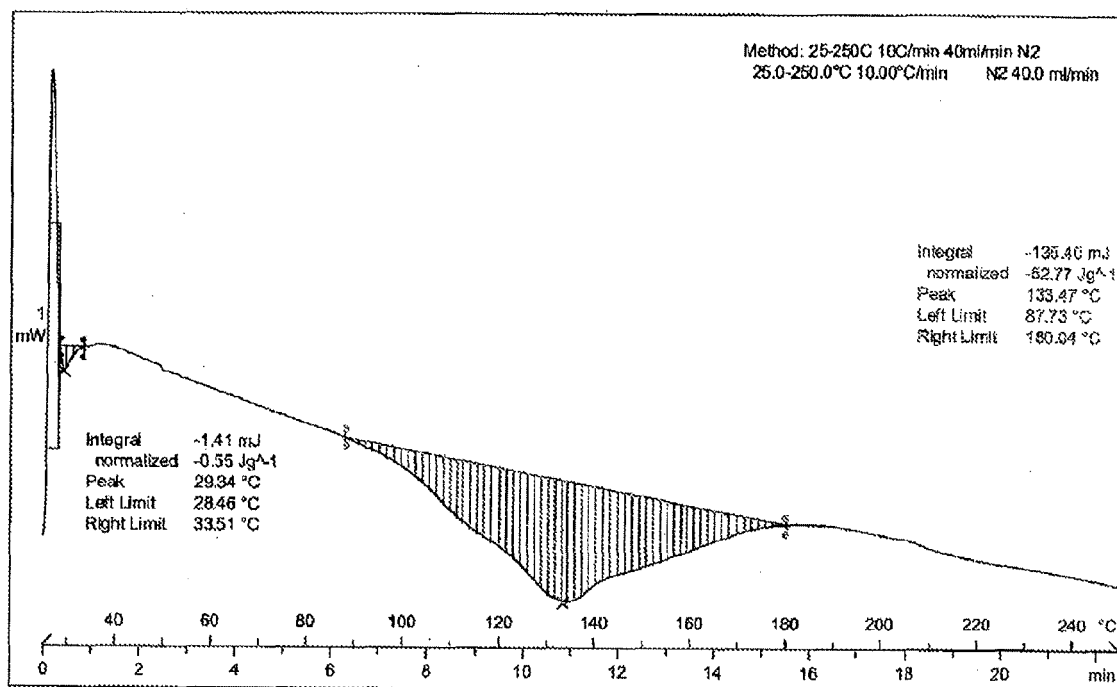
Figure 69: DSC thermogram of Dasatinib form AL
