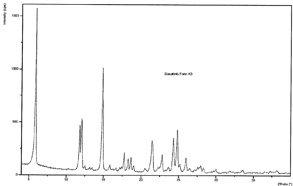
Figure 20: PXRD pattern of Dasatinib form K3
