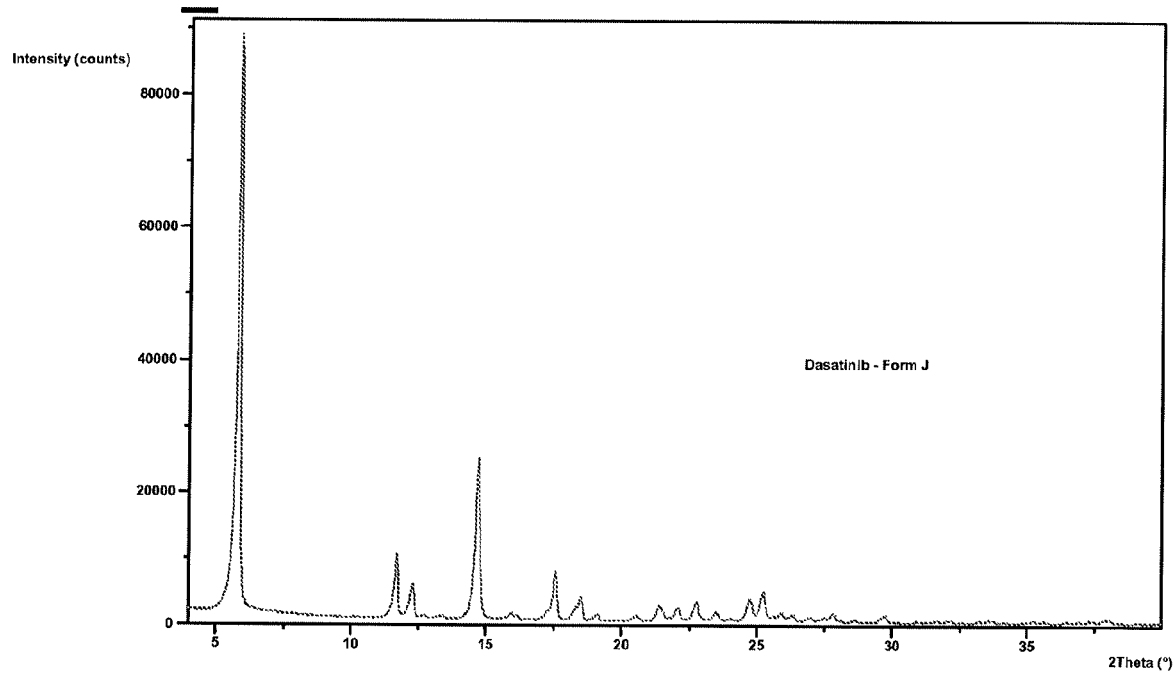
Figure 10: PXRD pattern of Dasatinib form J
