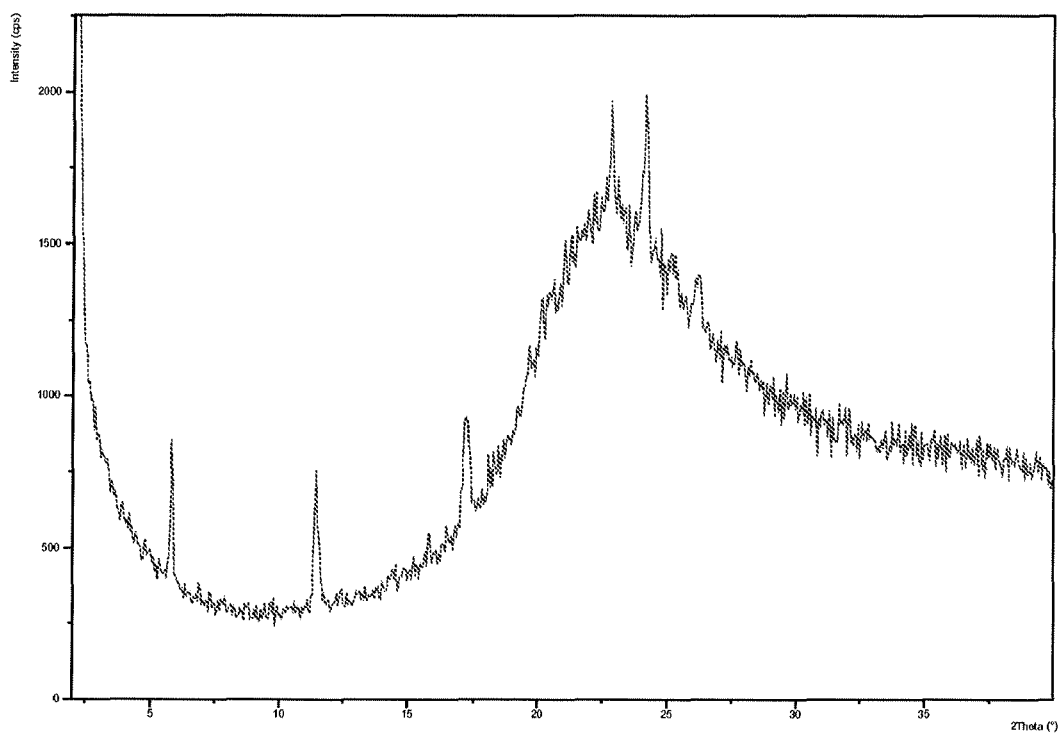
Figure 35: PXRD pattern of Dasatinib form AK
