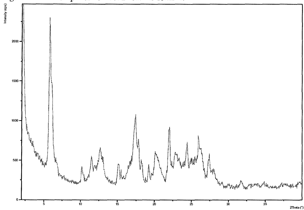
Figure 107: PXRD pattern of wet Dasatinib form AJ
