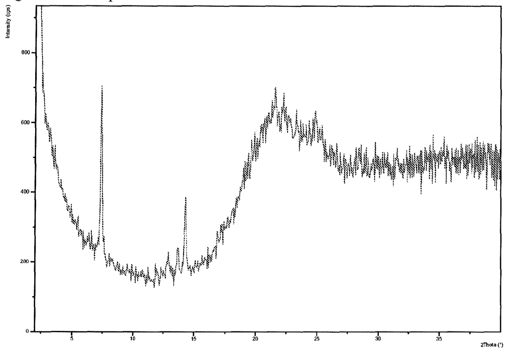
Figure 99: PXRD pattern of Dasatinib form BC
