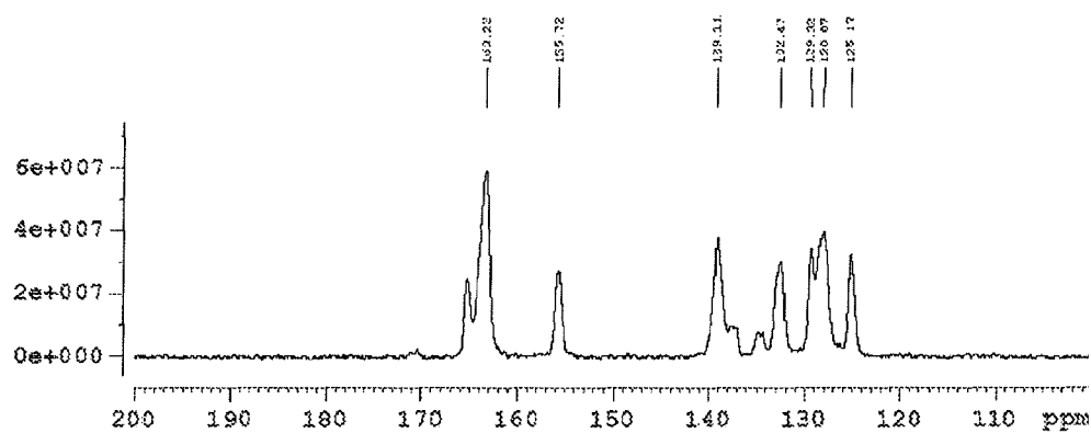
Figure 121: A full-width solid state ^{13}\text{C} NMR spectrum of dasatinib form A3.
