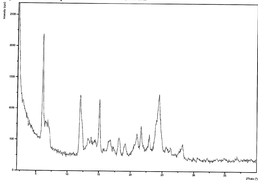
Figure 109: PXRD pattern of Dasatinib form BD
