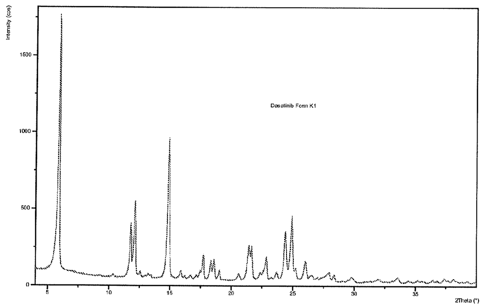
Figure 19: PXRD pattern of Dasatinib form K1
