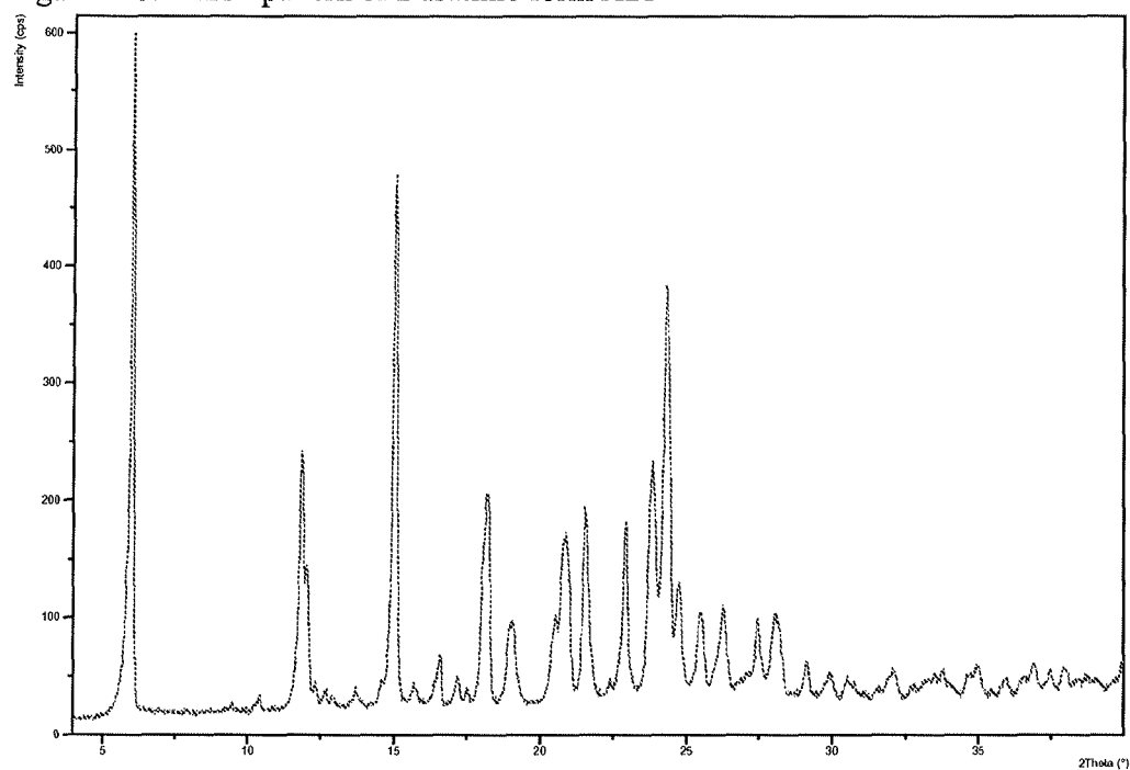
Figure 118: PXRD pattern of Dasatinib form A21
