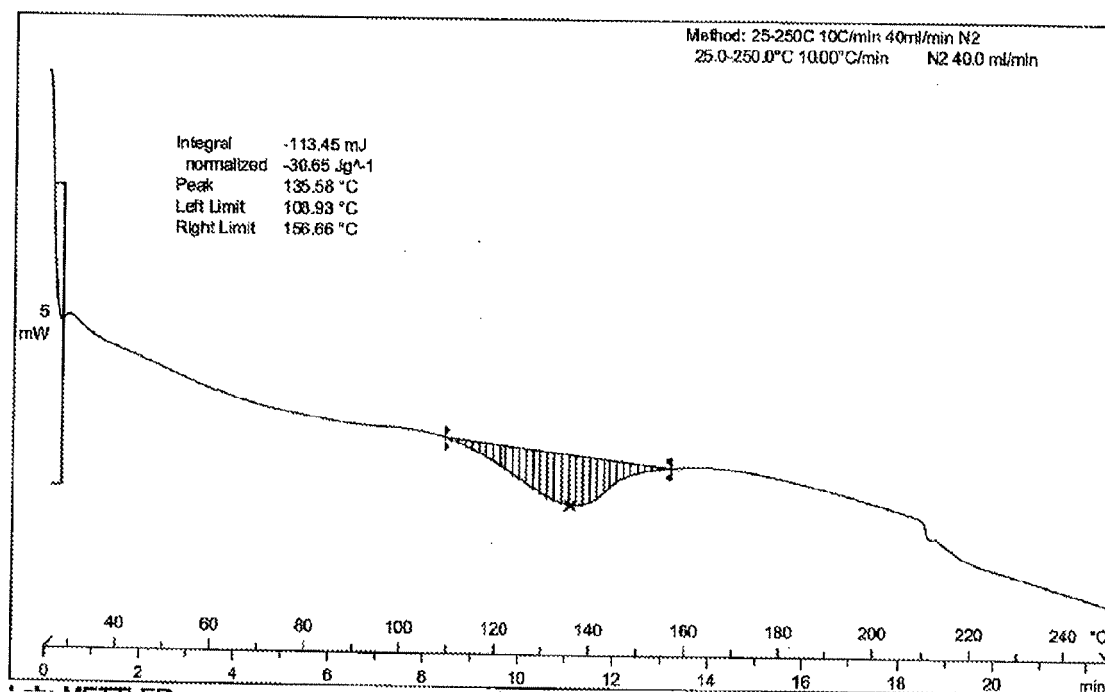
Figure 56: DSC thermogram of Dasatinib form AD
