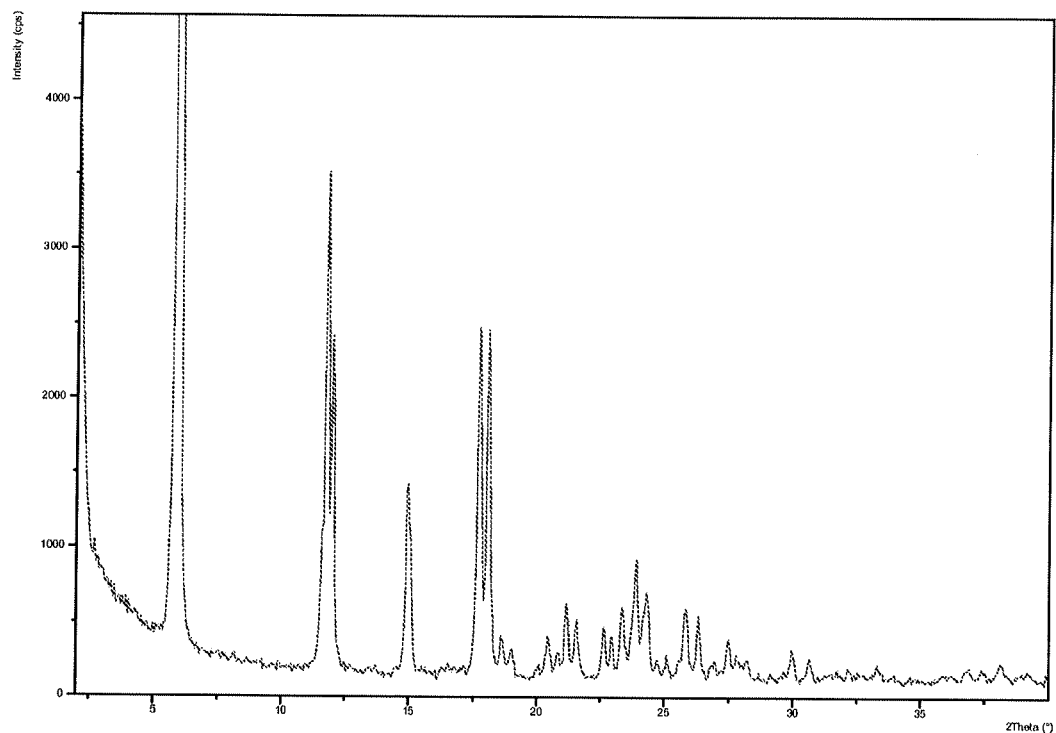
Figure 39: PXRD pattern of Dasatinib form AP
