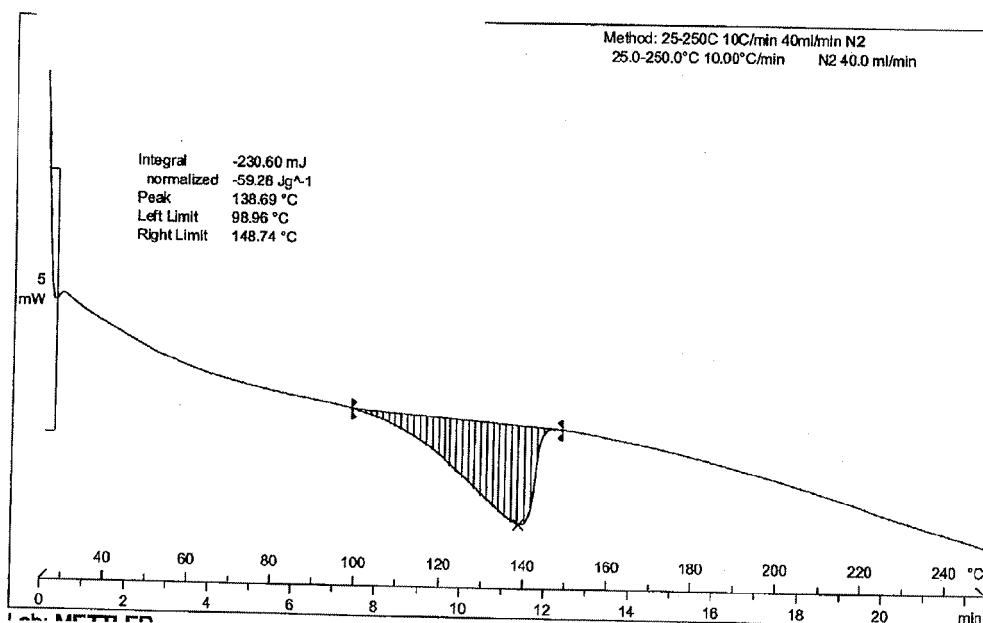
Figure 75: DSC thermogram of Dasatinib form AP
