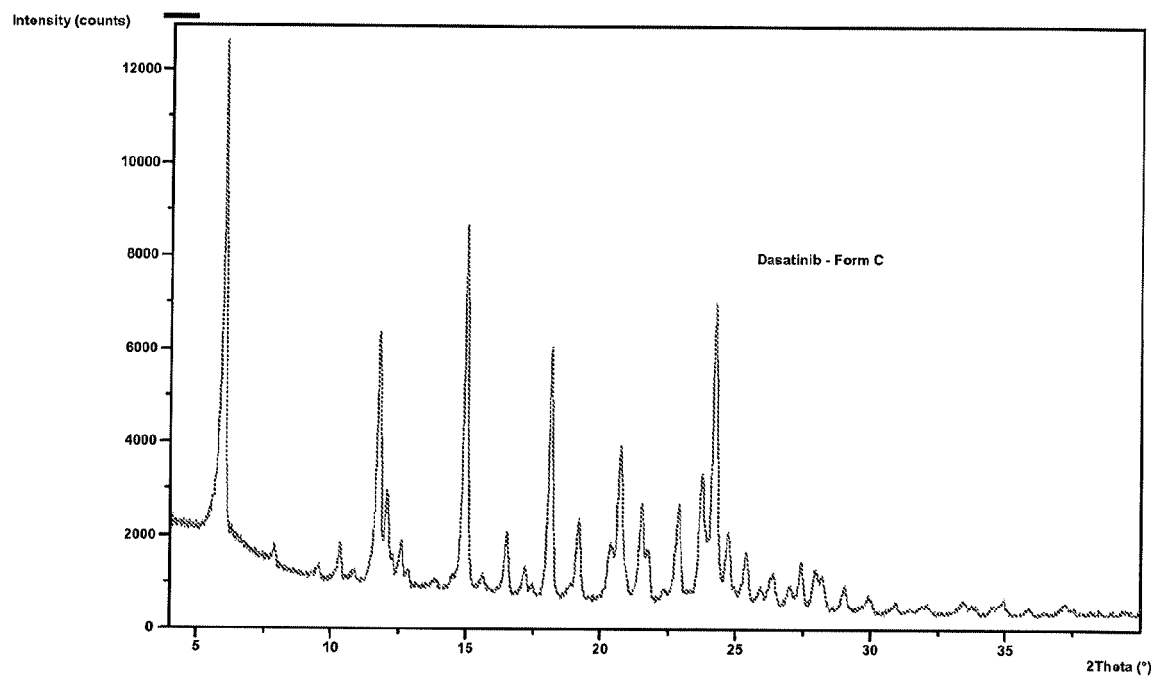
Figure 3: PXRD pattern of Dasatinib form C
