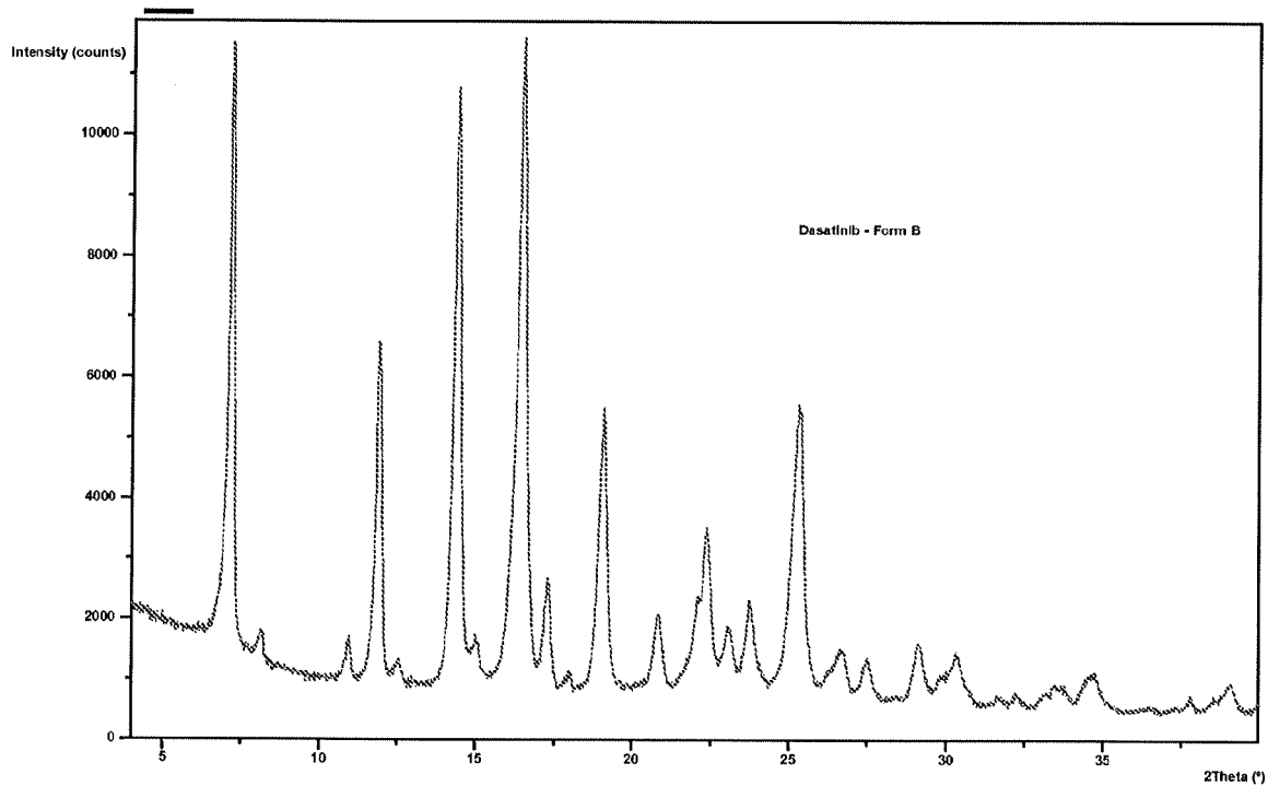
Figure 2: PXRD pattern of Dasatinib form B
