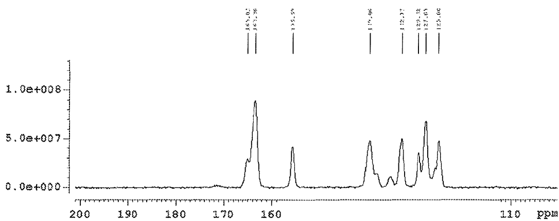
Figure 124: A detailed solid state ^{13}\text{C} NMR spectrum of dasatinib form A21.
