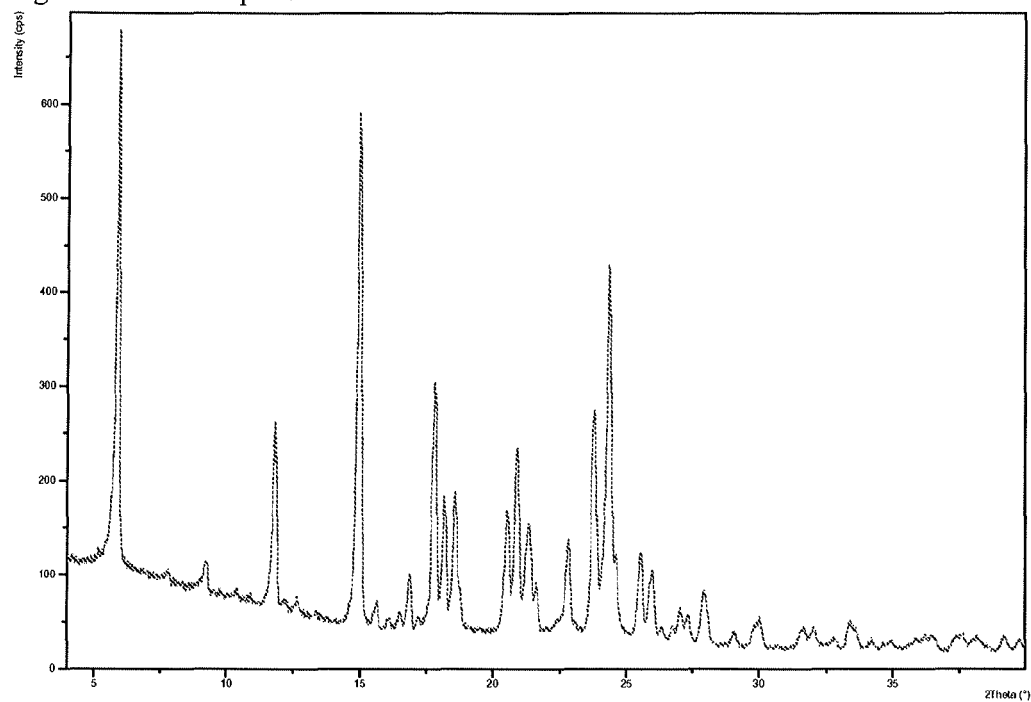
Figure 125: PXRD pattern of dasatinib form BL
