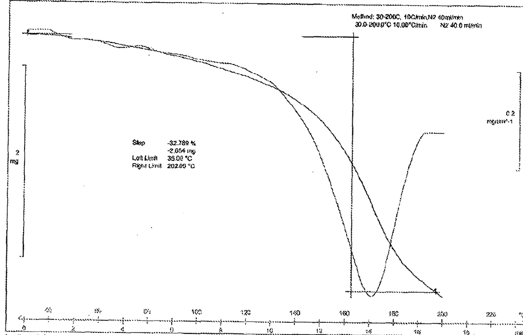
Figure 104: TGA thermogram of Dasatinib form BC
