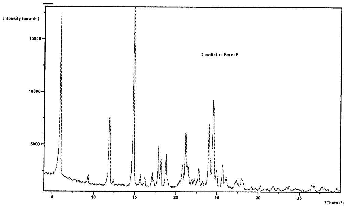
Figure 6: PXRD pattern of Dasatinib form F
