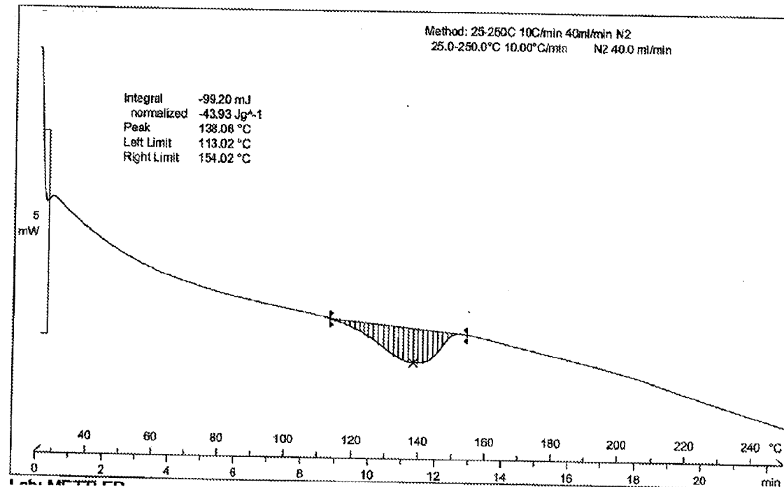
Figure 59: DSC thermogram of Dasatinib form AF
