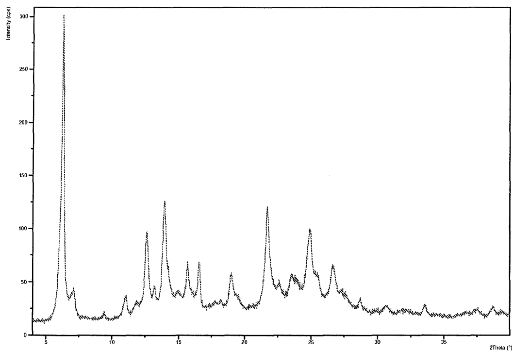
Figure 131: A powder XRD pattern of Dasatinib form BM
