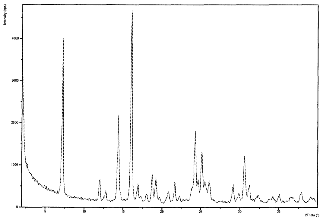
Figure 31: PXRD pattern of Dasatinib form AF
