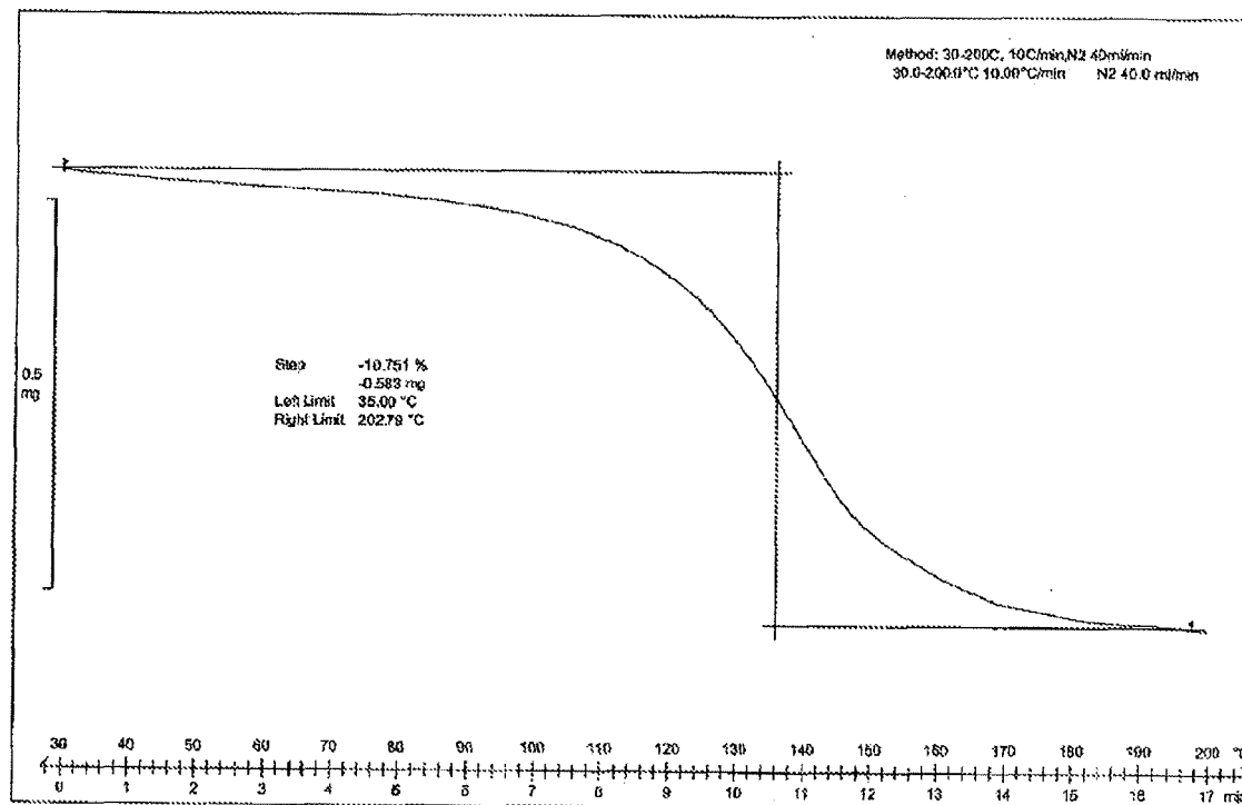
Figure 68: TGA thermogram of Dasatinib form AL
