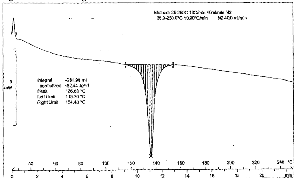
Figure 81: DSC thermogram of Dasatinib form AS
