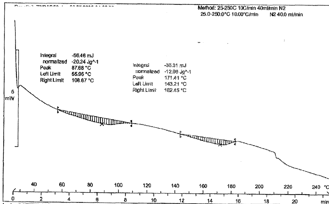
Figure 61: DSC thermogram of Dasatinib form AG
