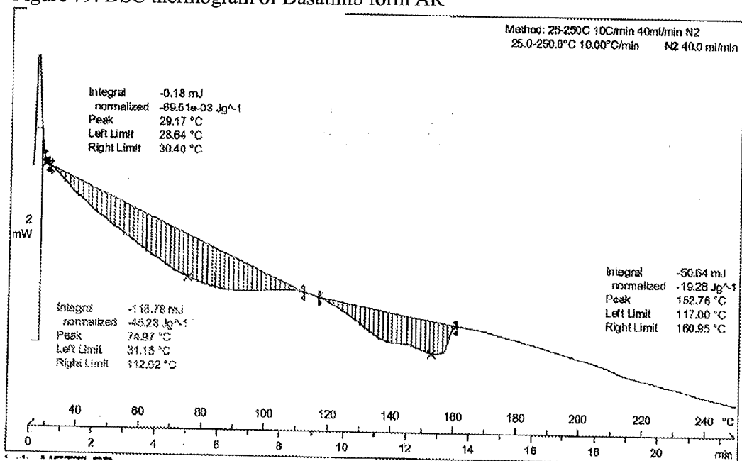
Figure 79: DSC thermogram of Dasatinib form AR
