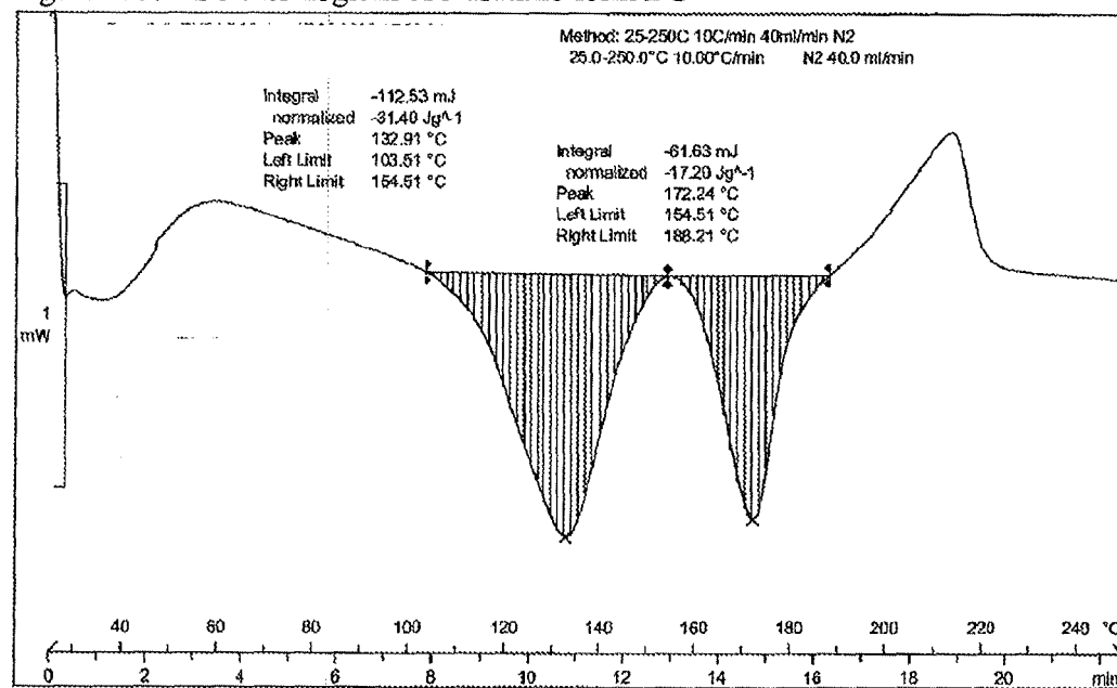
Figure 115: DSC thermogram of Dasatinib form BG
