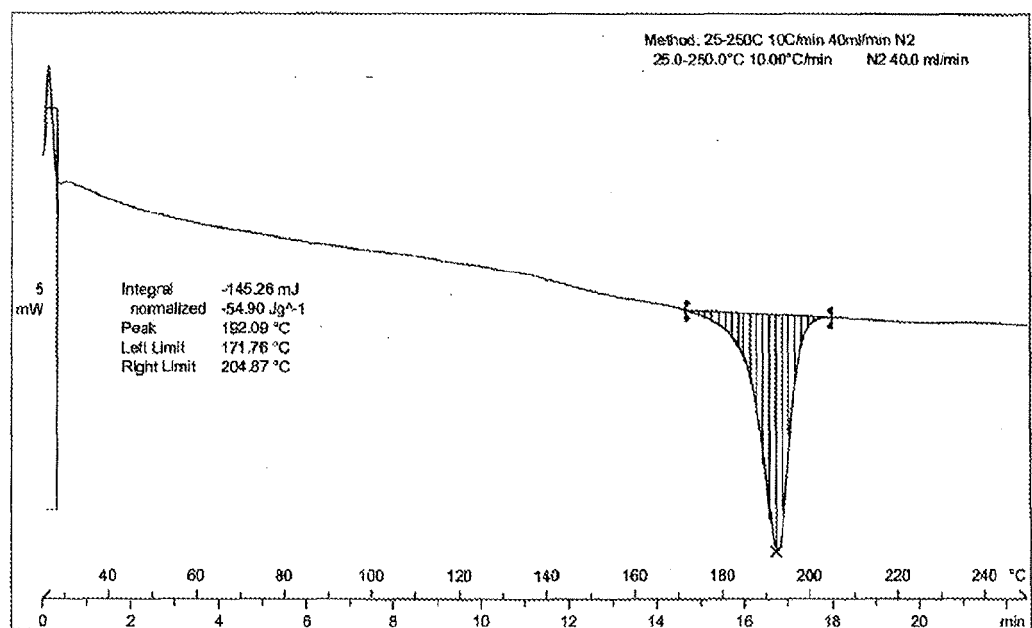
Figure 101: DSC thermogram of Dasatinib form BA
