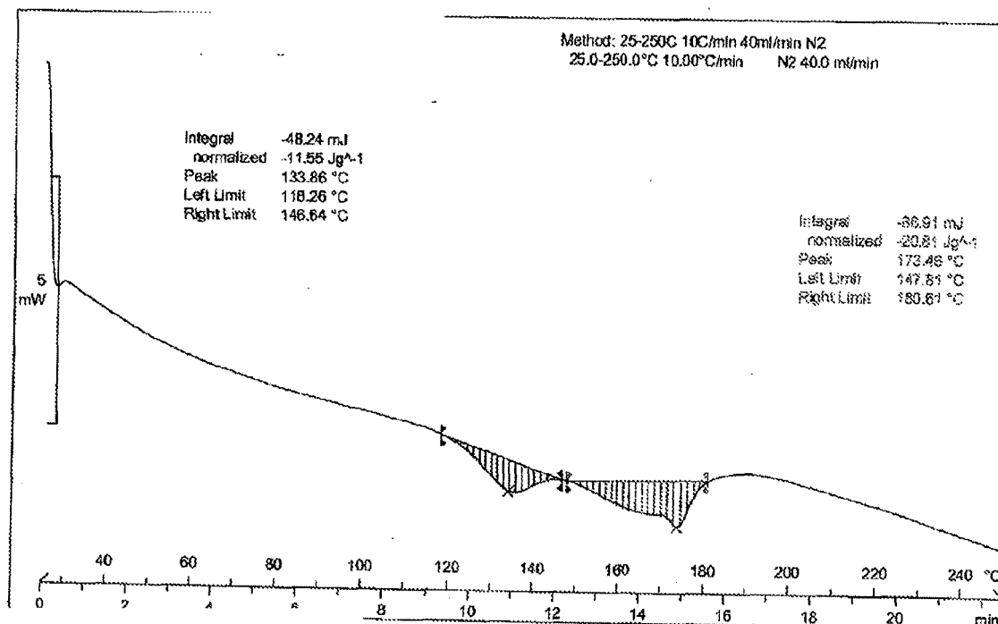
Figure 73: DSC thermogram of Dasatinib form AN
