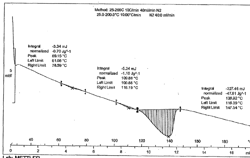
Figure 52: DSC thermogram of Dasatinib form AB
