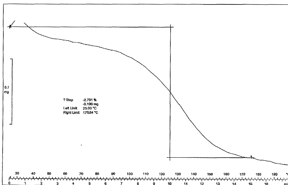
Figure 57: TGA thermogram of Dasatinib form AE
