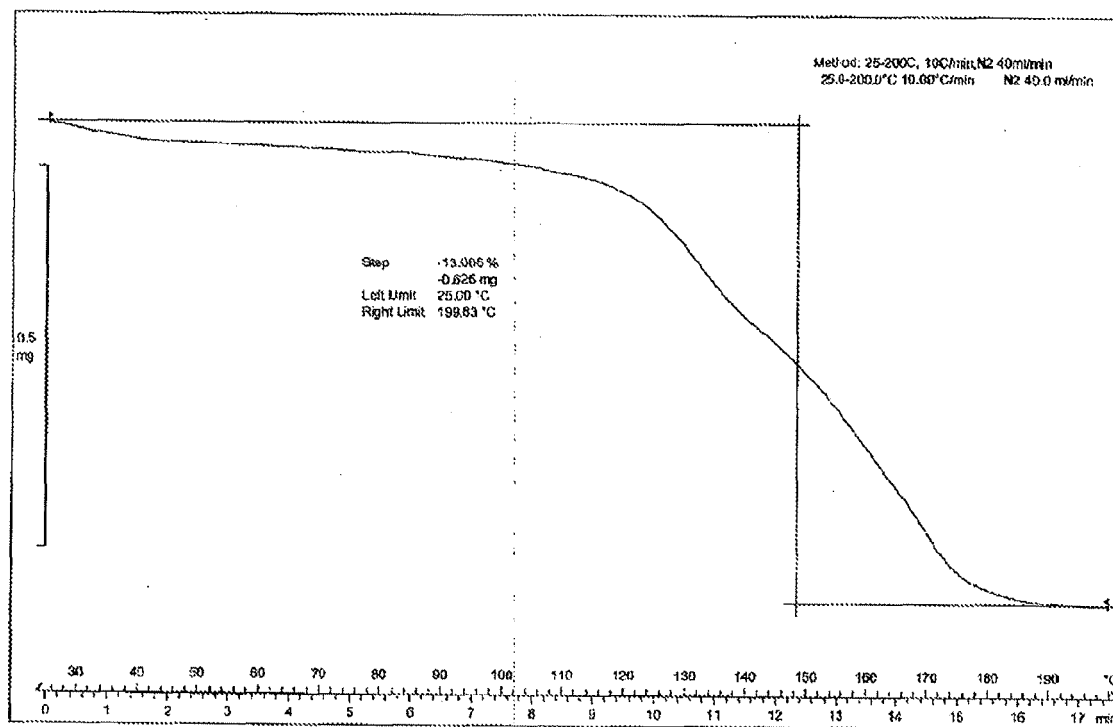
Figure 72: TGA thermogram of Dasatinib form AN
