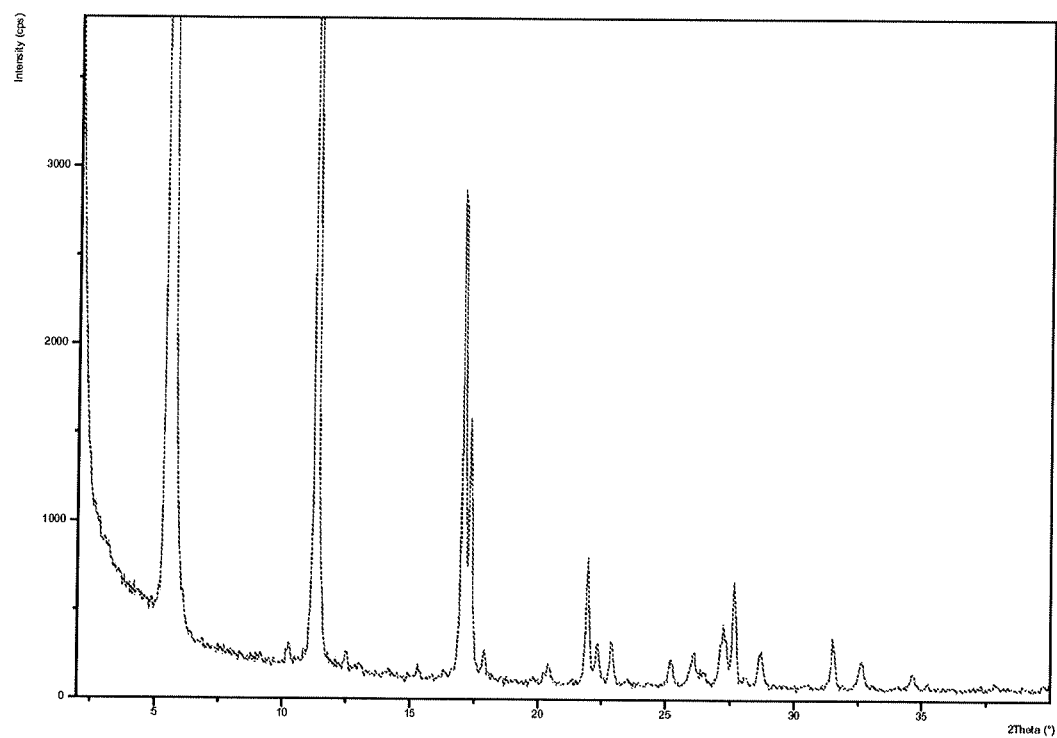
Figure 33: PXRD pattern of Dasatinib form AI
