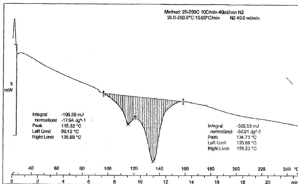
Figure 85: DSC thermogram of Dasatinib form AU
