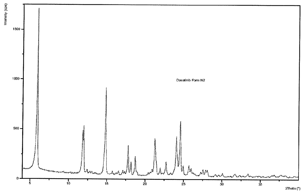
Figure 23: PXRD pattern of Dasatinib form N2
