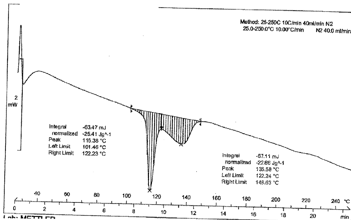
Figure 65: DSC thermogram of Dasatinib form AJ
