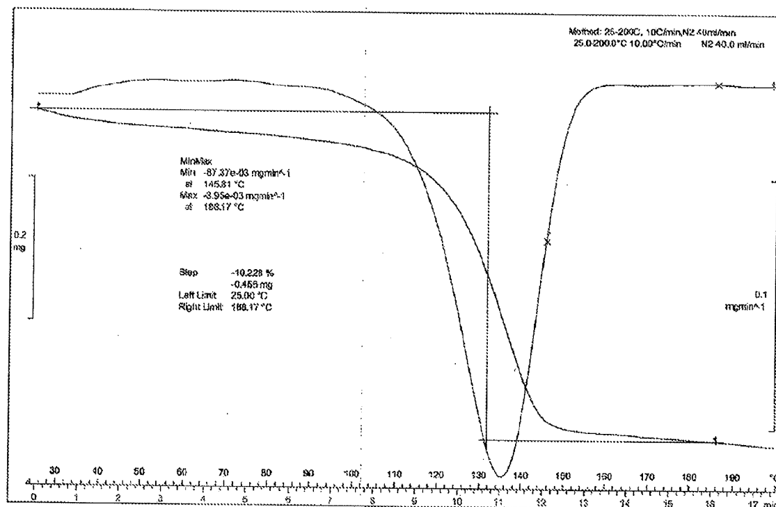
Figure 58: TGA thermogram of Dasatinib form AF
