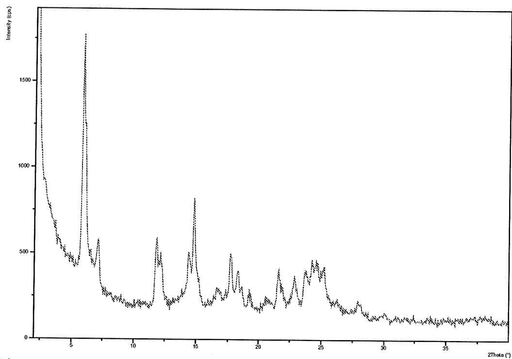
Figure 37: PXRD pattern of Dasatinib form AM
