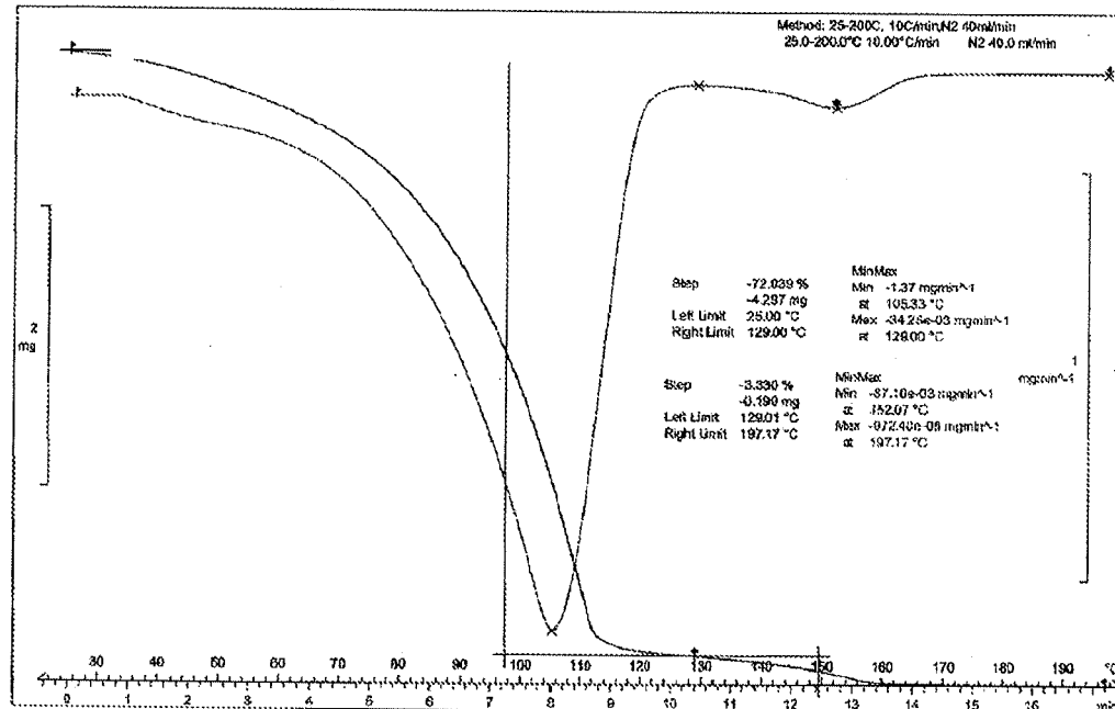
Figure 94: TGA thermogram of Dasatinib form AH
