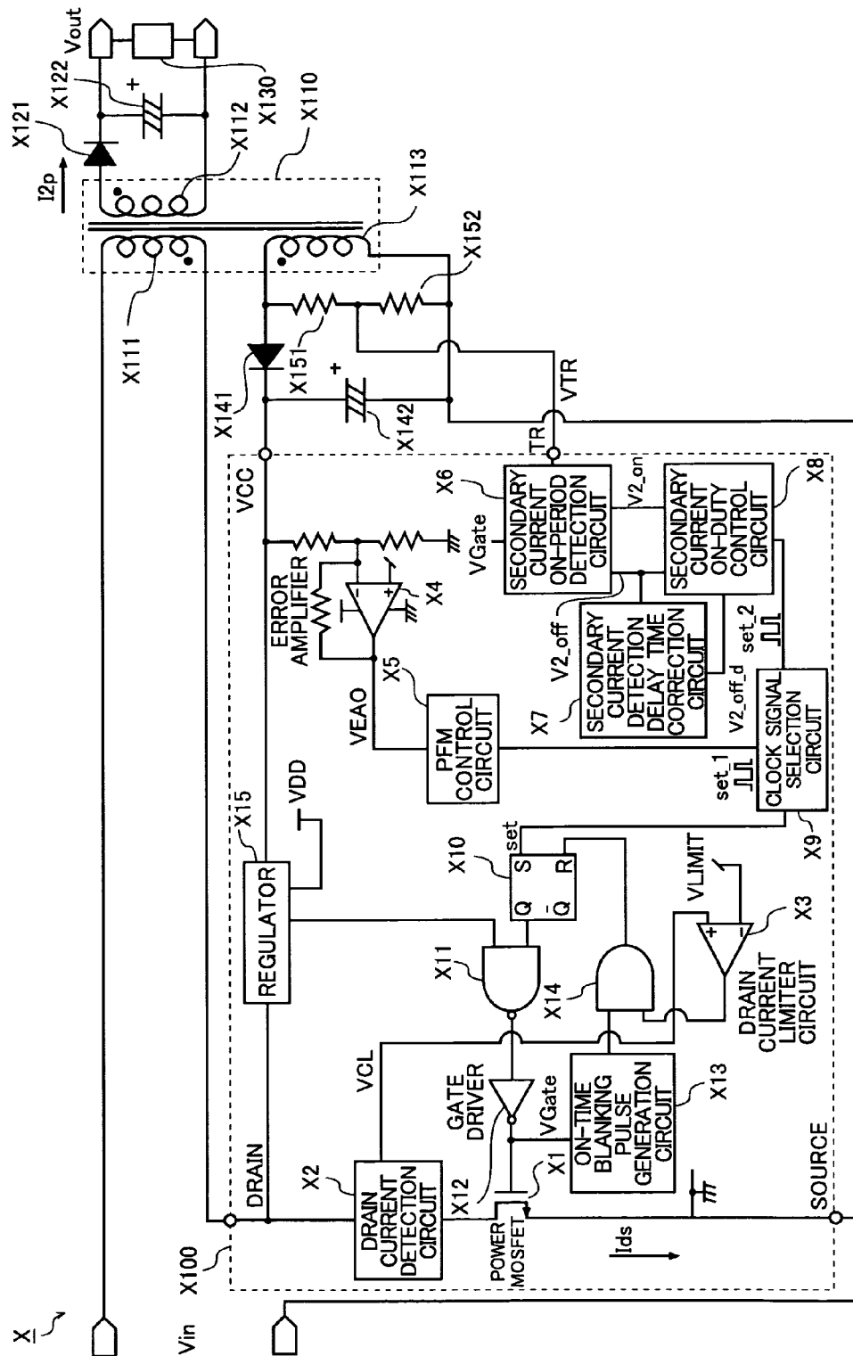
FIG. 11 Related Art
