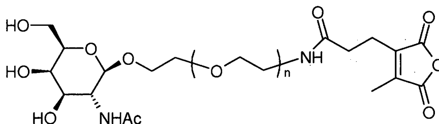
CDM-NAG
