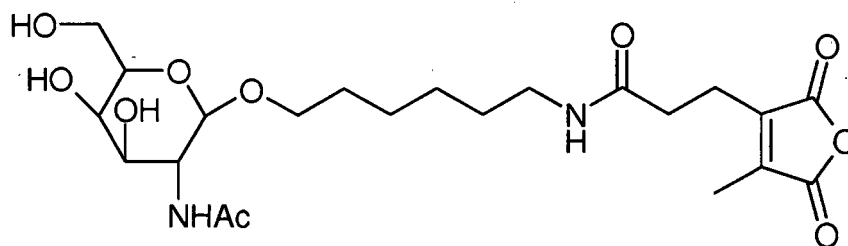
CDM-NAG with alkyl spacer
