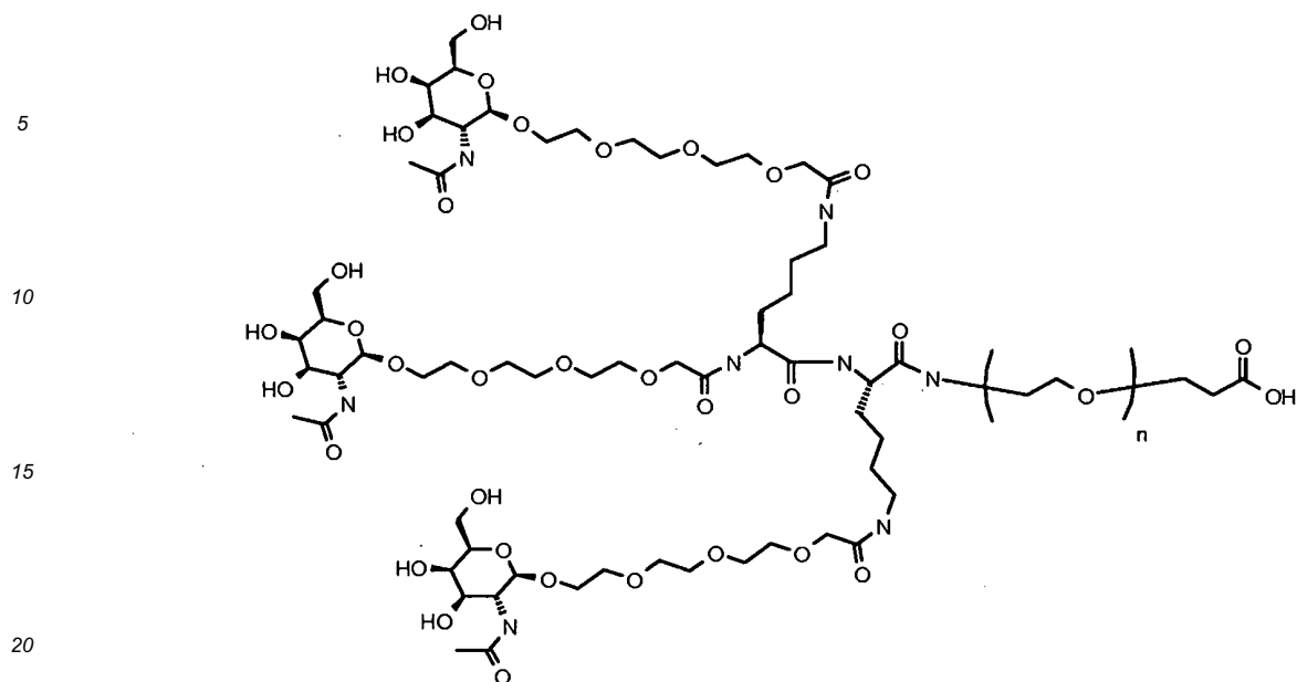
Galactose cluster with PEG spacer; targeting ligand attached to the siRNA through the carboxyl group.
