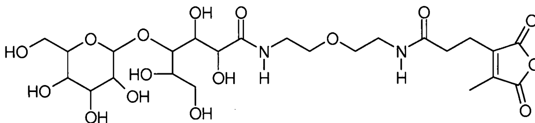
CDM-lactose
