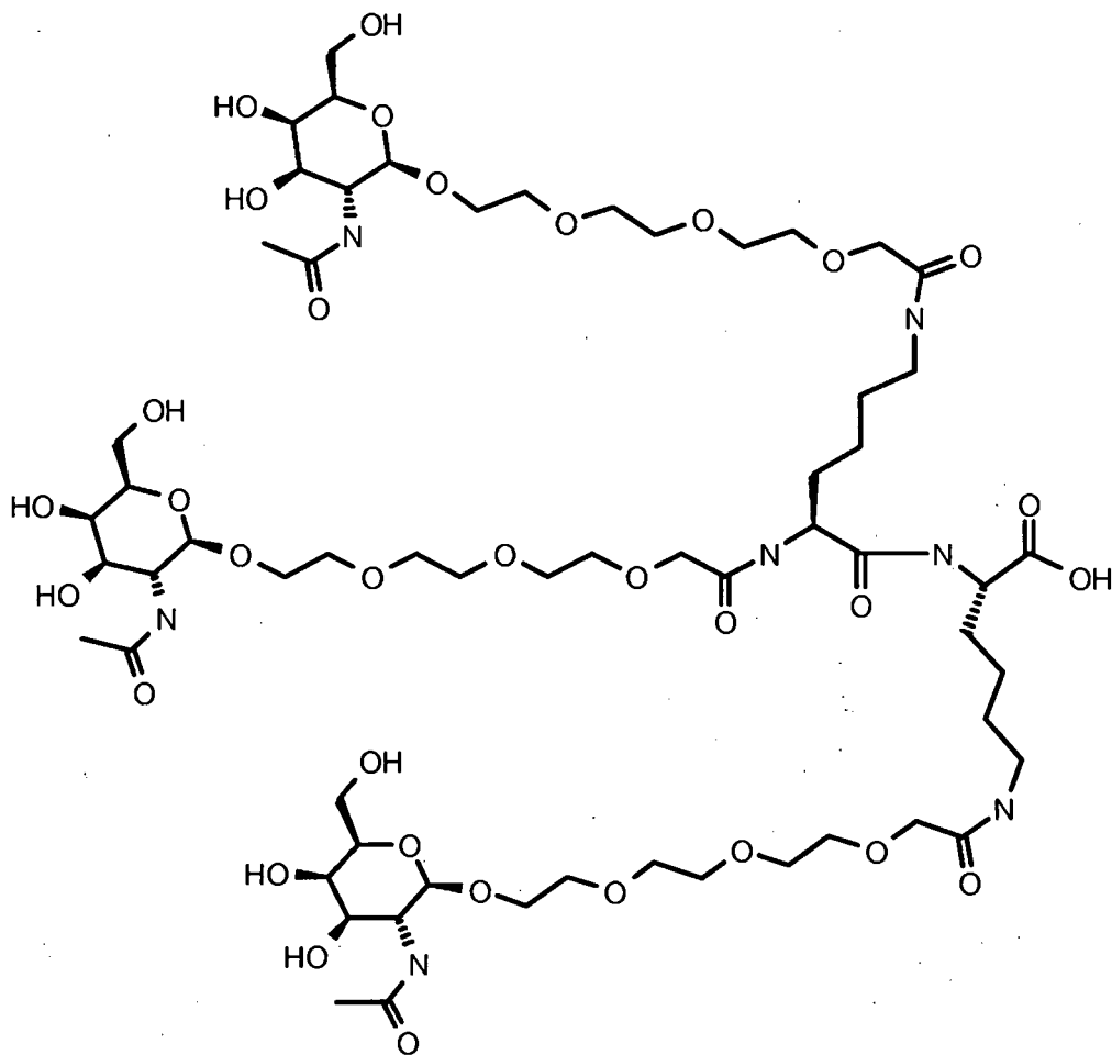
Galactose cluster without PEG spacer; targeting ligand attached to the siRNA through the carboxyl group.
