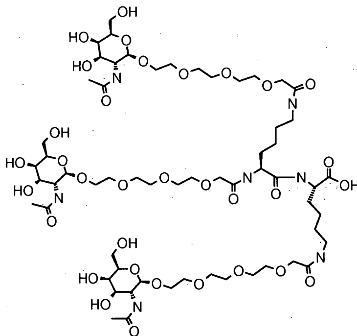
GalNAc Cluster
