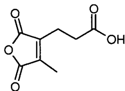
50 2-propionic-3-methylmaleic anhydride
