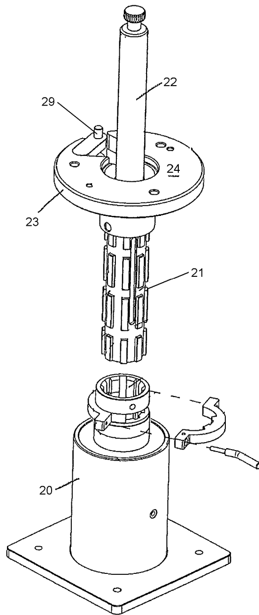
Fig. 3 (prior art)
