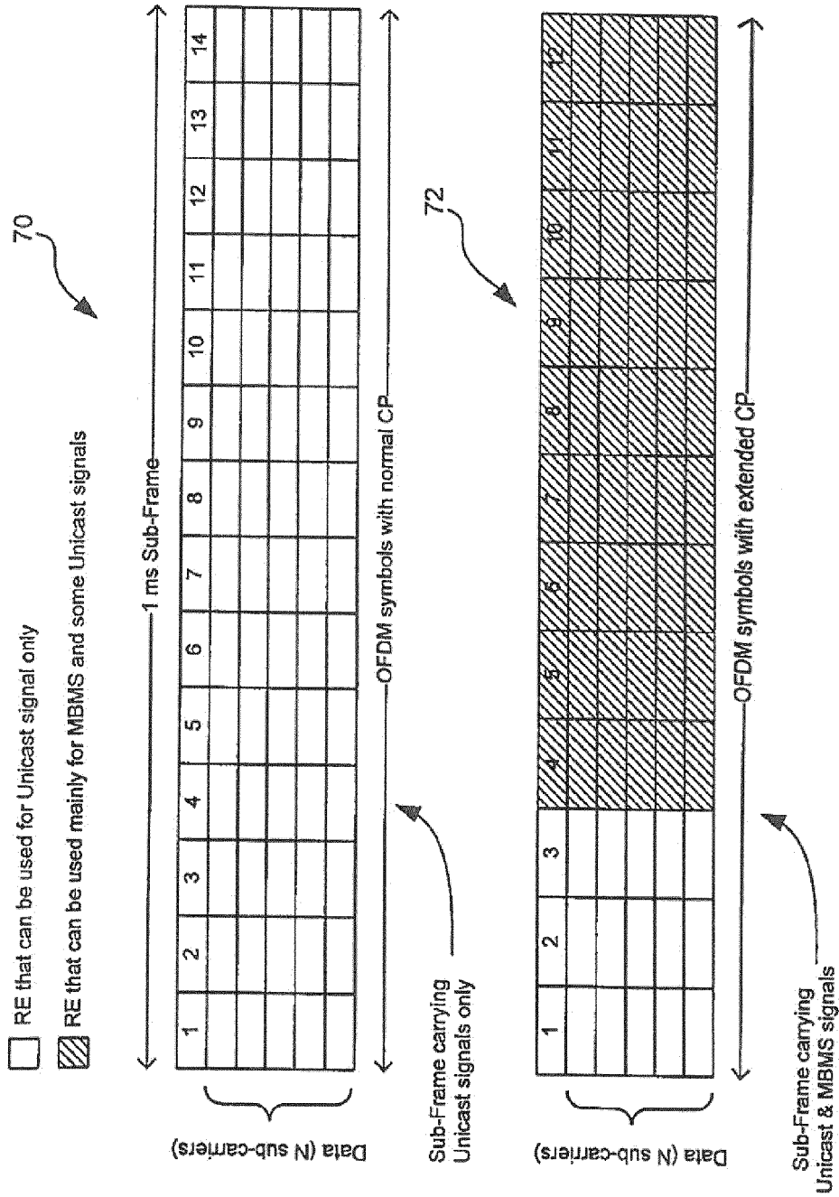
3GPP Assumed Sub-Frame Structure
