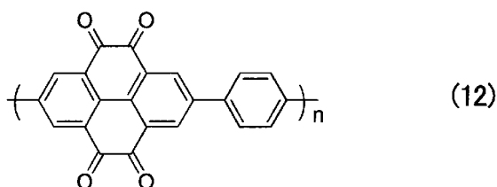
[Chemical Formula 20]
