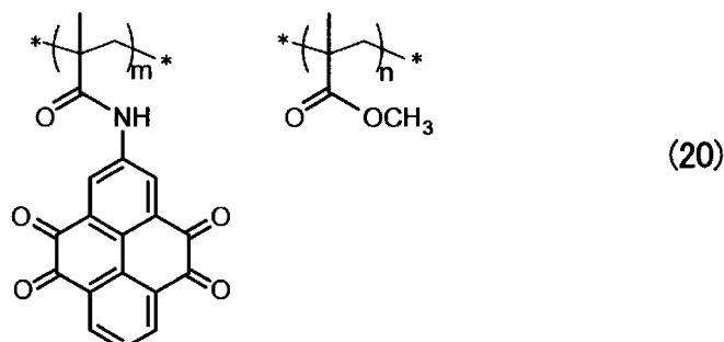
[Chemical Formula 28]
