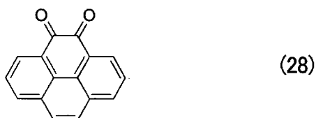
[Chemical Formula 36]
