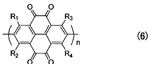
[Chemical Formula 14]
