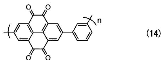
[Chemical Formula 22]
