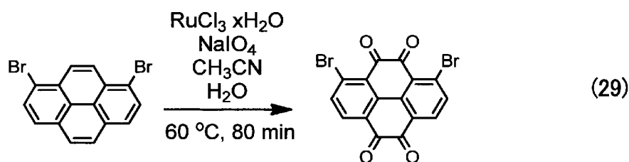
[Chemical Formula 37]
