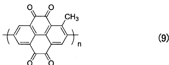
[Chemical Formula 17]
