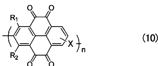
[Chemical Formula 18]
