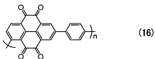
[Chemical Formula 24]
