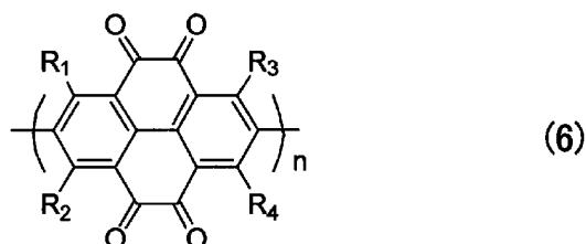
[Chemical Formula 2]
