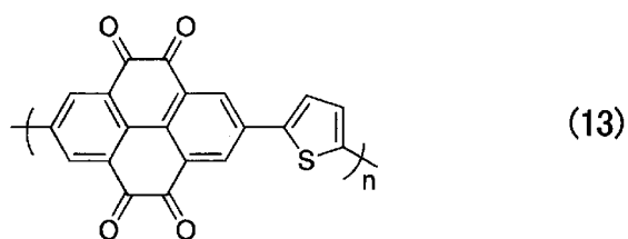
[Chemical Formula 21]
