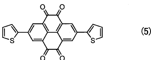
[Chemical Formula 13]
