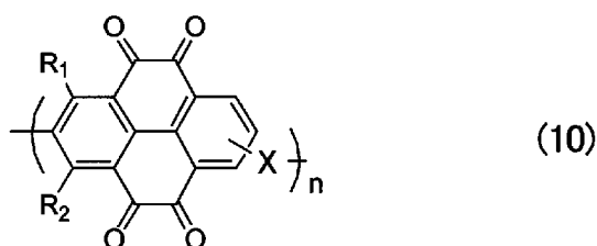
[Chemical formula 3]
