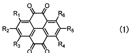
[Chemical Formula 1]
