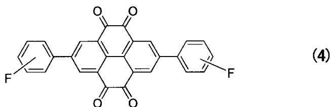
[Chemical Formula 12]
