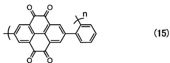
[Chemical Formula 23]
