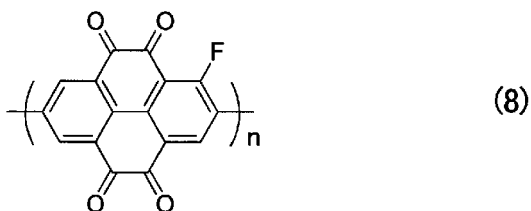
[Chemical Formula 16]
