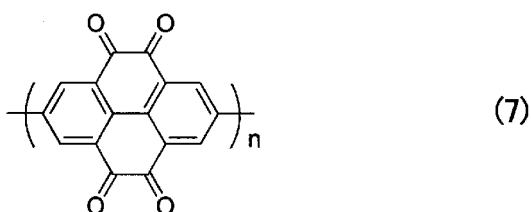
[Chemical Formula 15]
