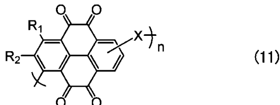
[Chemical Formula 19]
