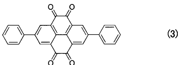
[Chemical Formula 11]
