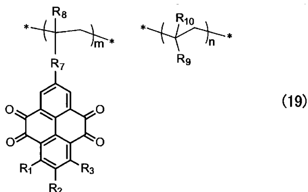
[Chemical Formula 4]
