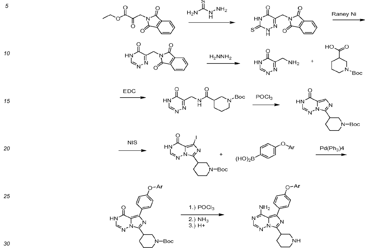
Scheme II.
