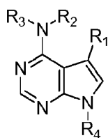
Formula (A2),
