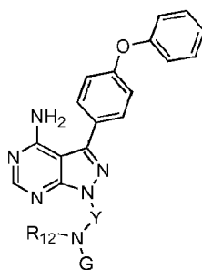
Formula (C1),
