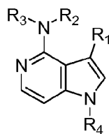
Formula (A6)
