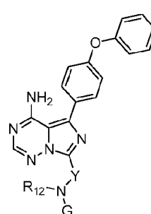
Formula (C4),
