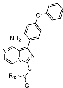
Formula (C5),
