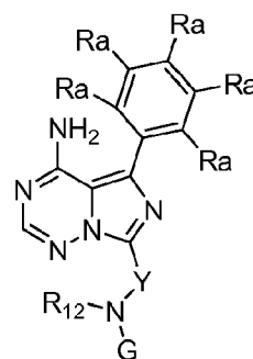
Formula (B3),
