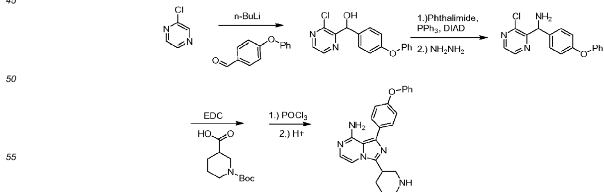
Scheme III
