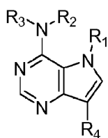
Formula (A3),
