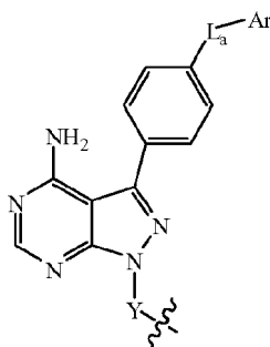
Formula (II)
