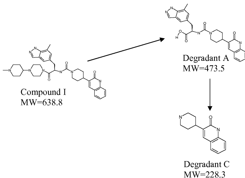
Scheme 6.
