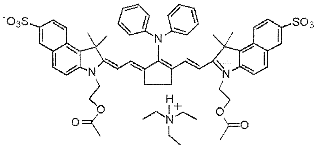
Infrared absorbing dye (2)
