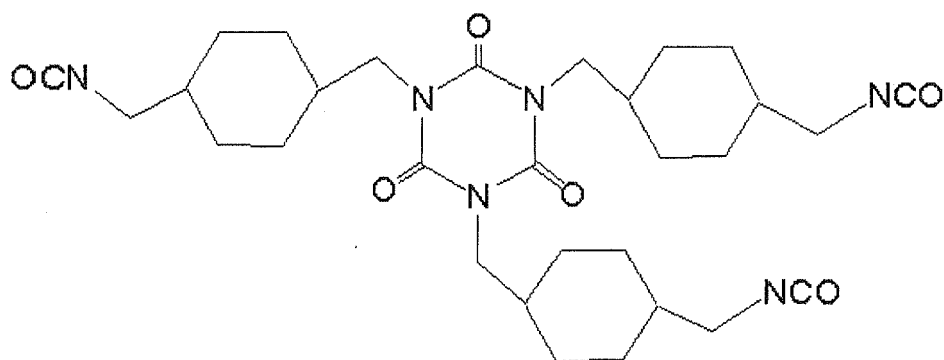
Polyfunctional isocyanate
