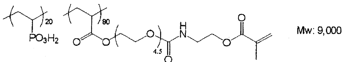
Polymer (SP2)
