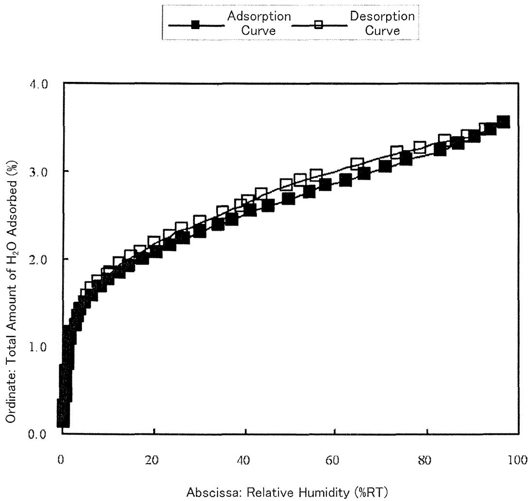
Isothermal Water Vapor Adsorption-Desorption Curve of Br 2
