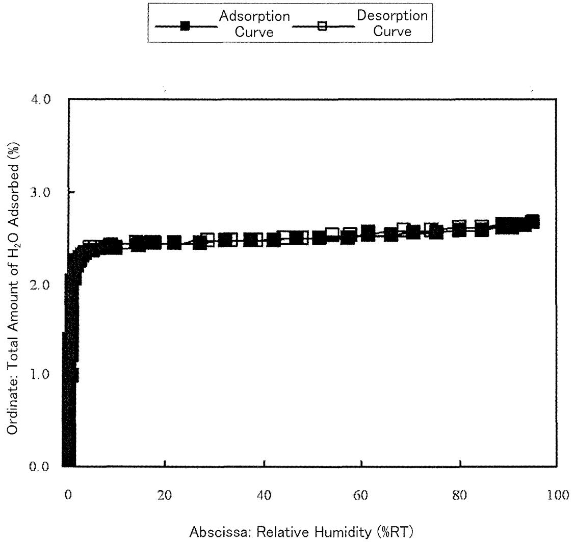
Isothermal Water Vapor Adsorption-Desorption Curve of CI 1
