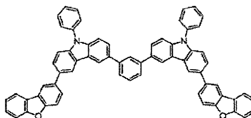
Compound (H2)
