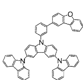
Compound (32)
