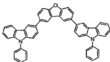
Compound (H4)
