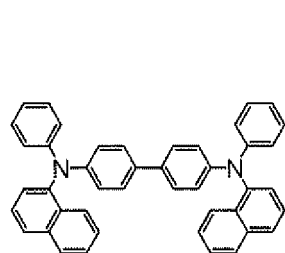
Compound (HT)
