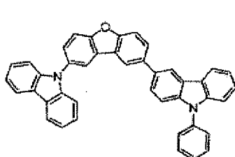
Compound (H5)
