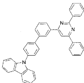
Compound (HB)
