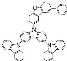
Compound (2)
