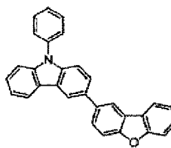
Compound (H6)
