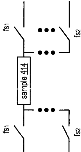
FIG. 109A sample & hold circuit 204
