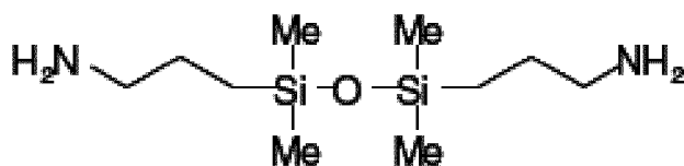
1,2-bis(3-aminopropyl)-tetramethyldisiloxane
