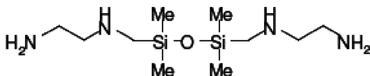
and 1,2-bis(2-aminoethylaminomethyl)-tetramethyldisiloxane
