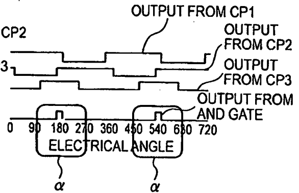
ABNORMAL STATE (PHASE DIFFERENCE: 90 DEGREES)
