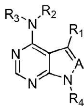
Formula (A1),
