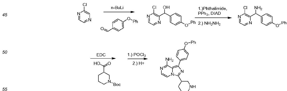
Scheme III
