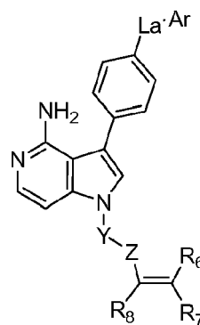
Formula (D6)
