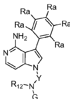
Formula (B6)
