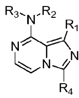
Formula (A5),
