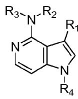
Formula (A6)
