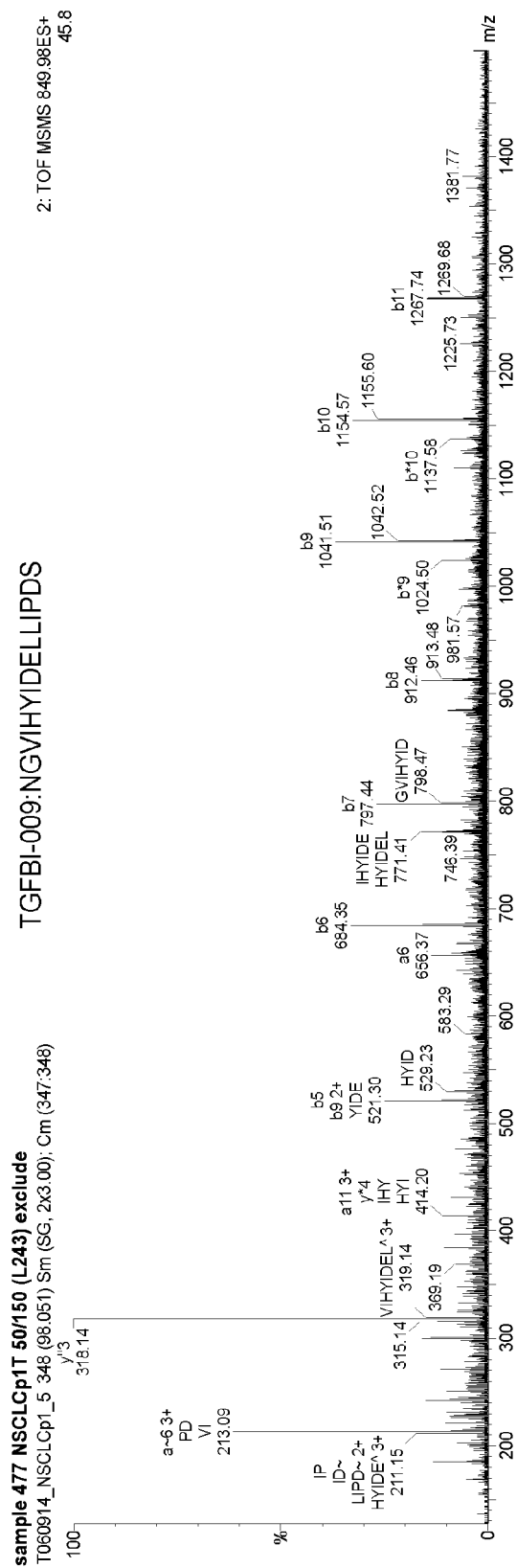
Figure 2e: TGFBI-009 (NSCLC-Pool 1)
