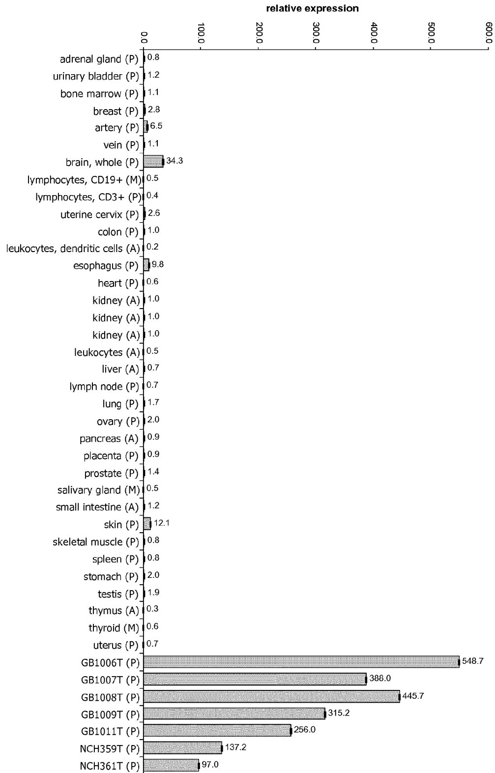
Figure 3a: Expression profile of PTP
