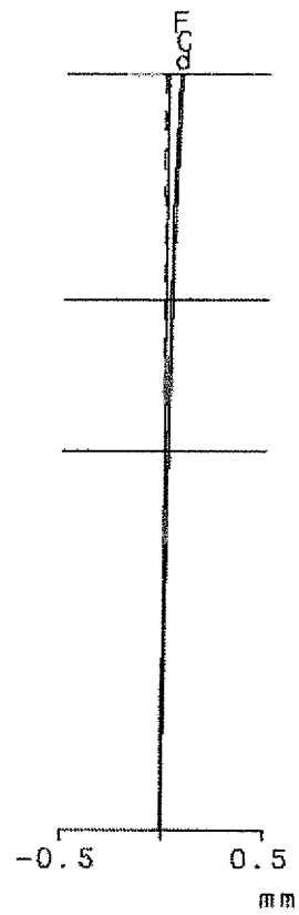
Spherical Aberration FN 6
