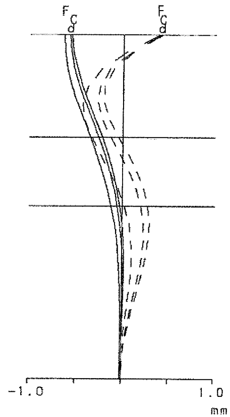
Astigmatism \omega 50^\circ
