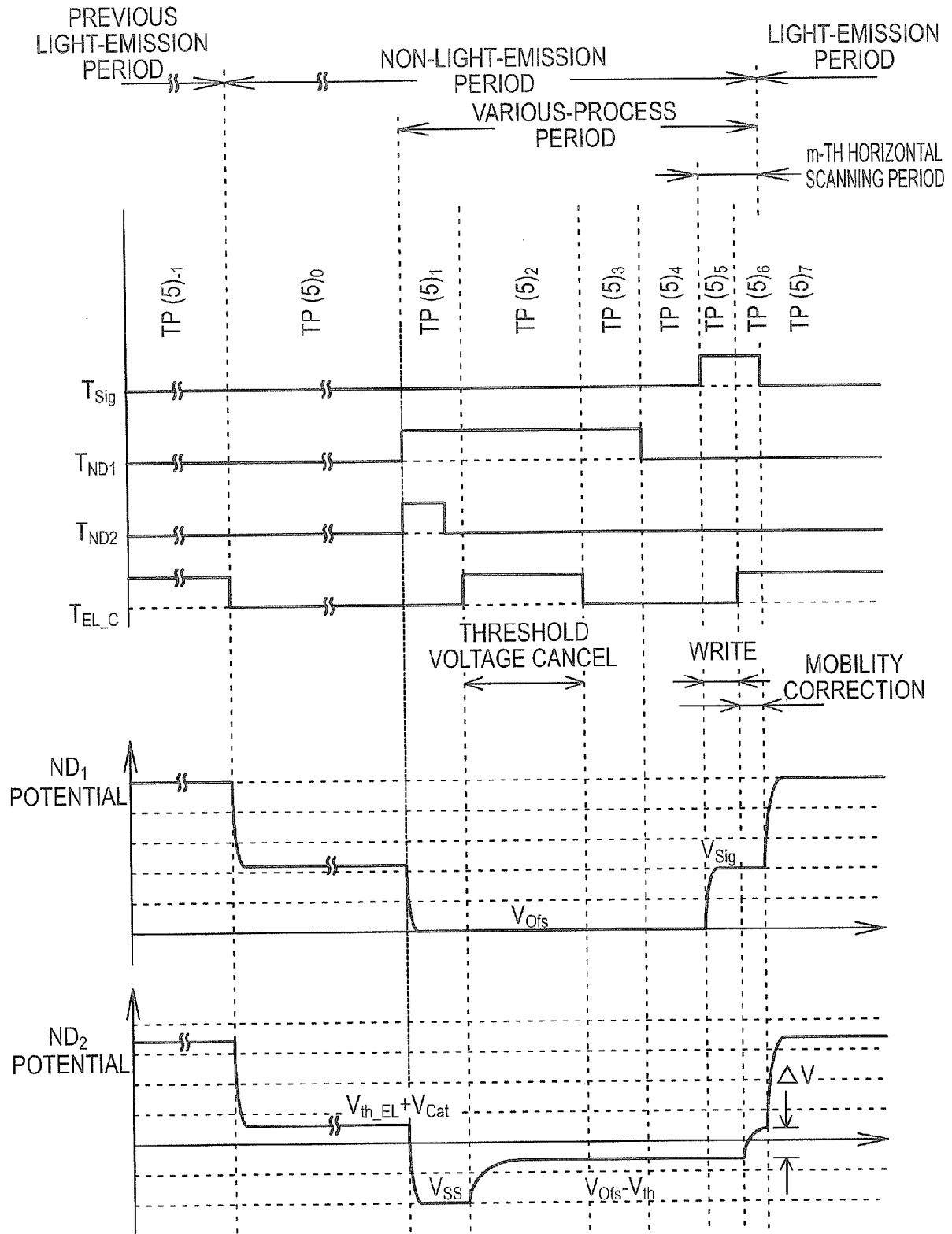
FIG. 6 [5Tr/1C DRIVING CIRCUIT]
