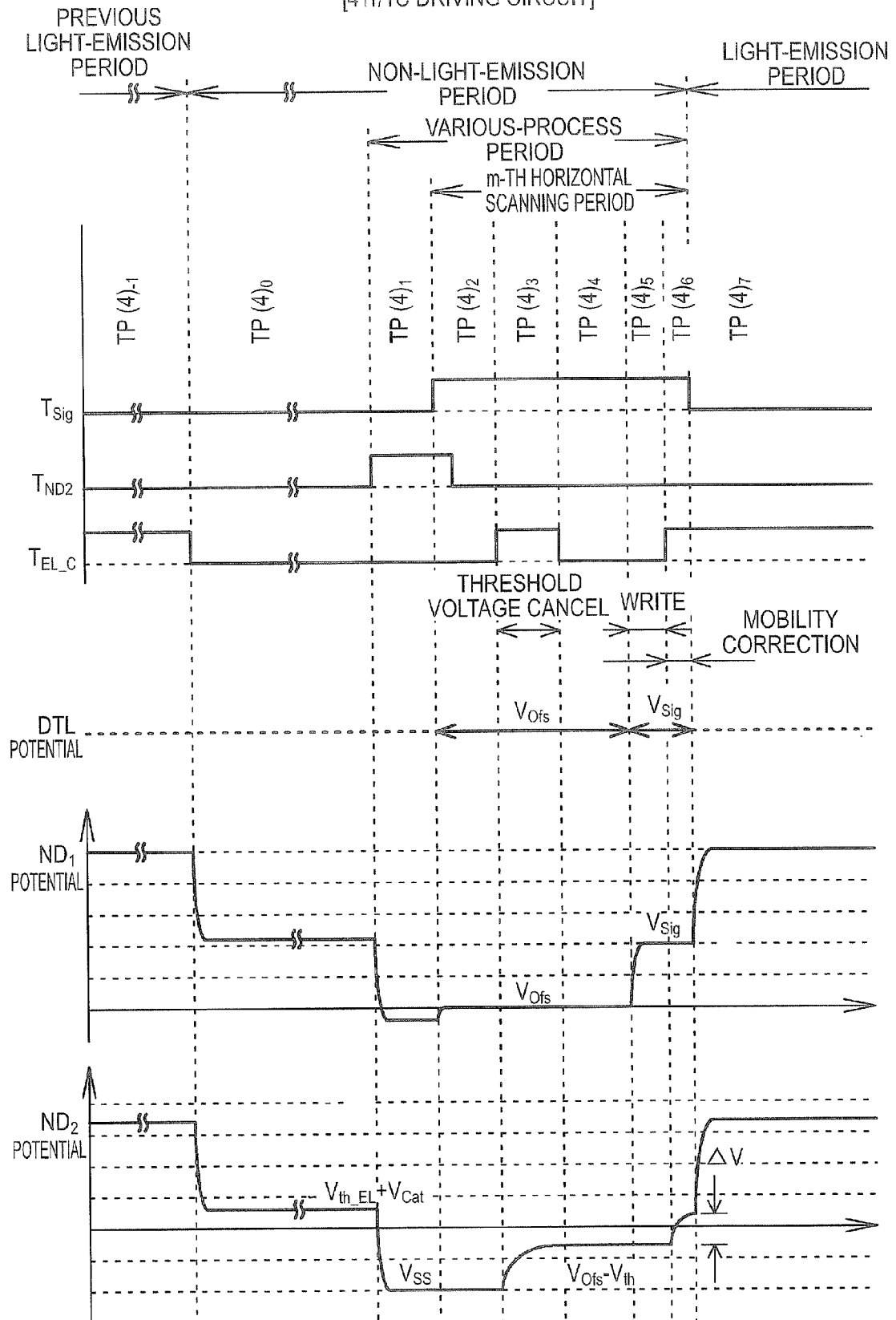
FIG. 11 [4Tr/1C DRIVING CIRCUIT]
