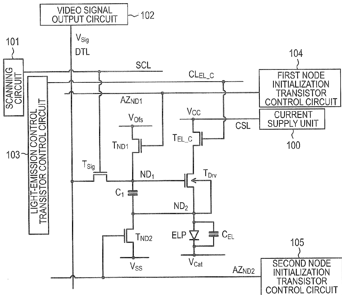
FIG.5 [5Tr/1C DRIVING CIRCUIT]
