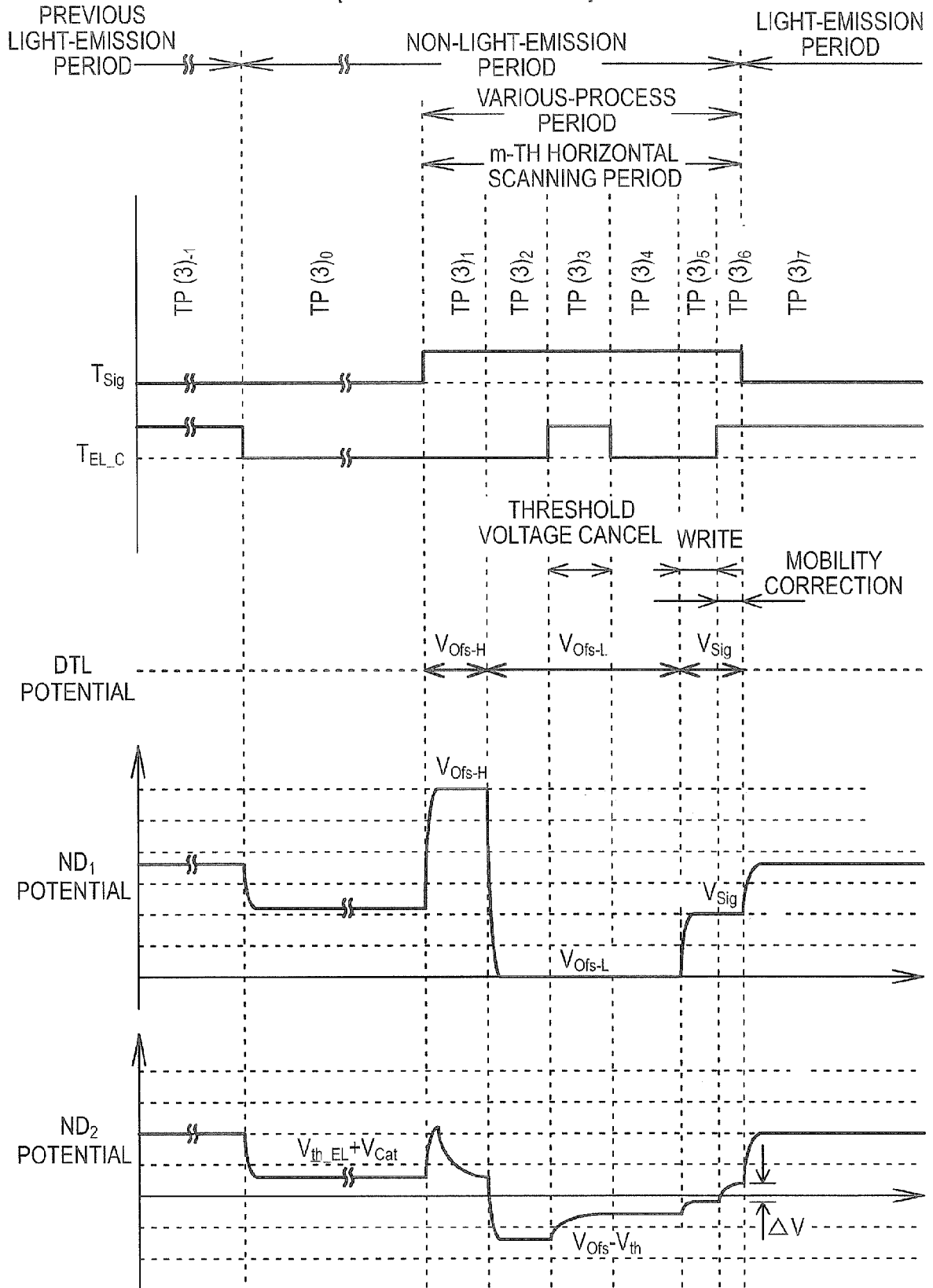
FIG. 16 [3Tr/1C DRIVING CIRCUIT]
