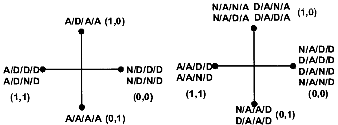
PUCCH resource 1,
