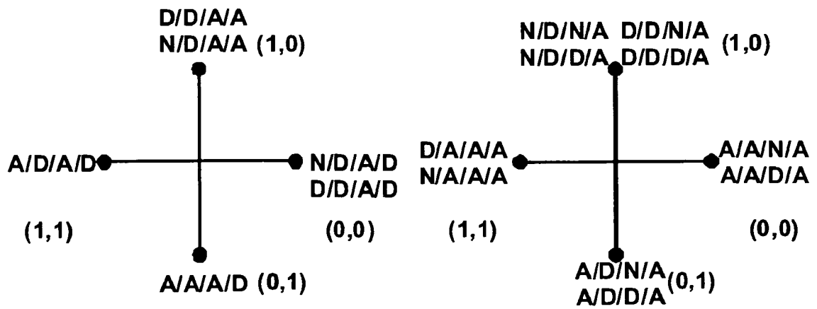
PUCCH resource 3,
