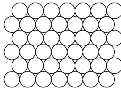
hexagonal packing
