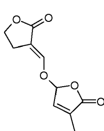
(II-22c)
