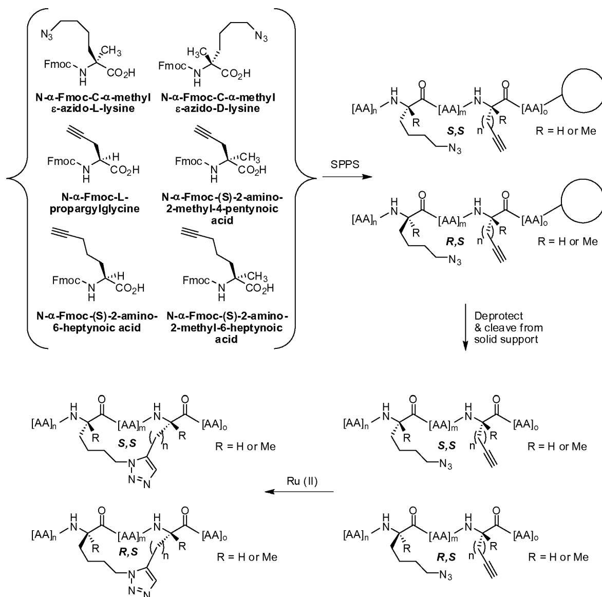
Synthetic Scheme 4:
