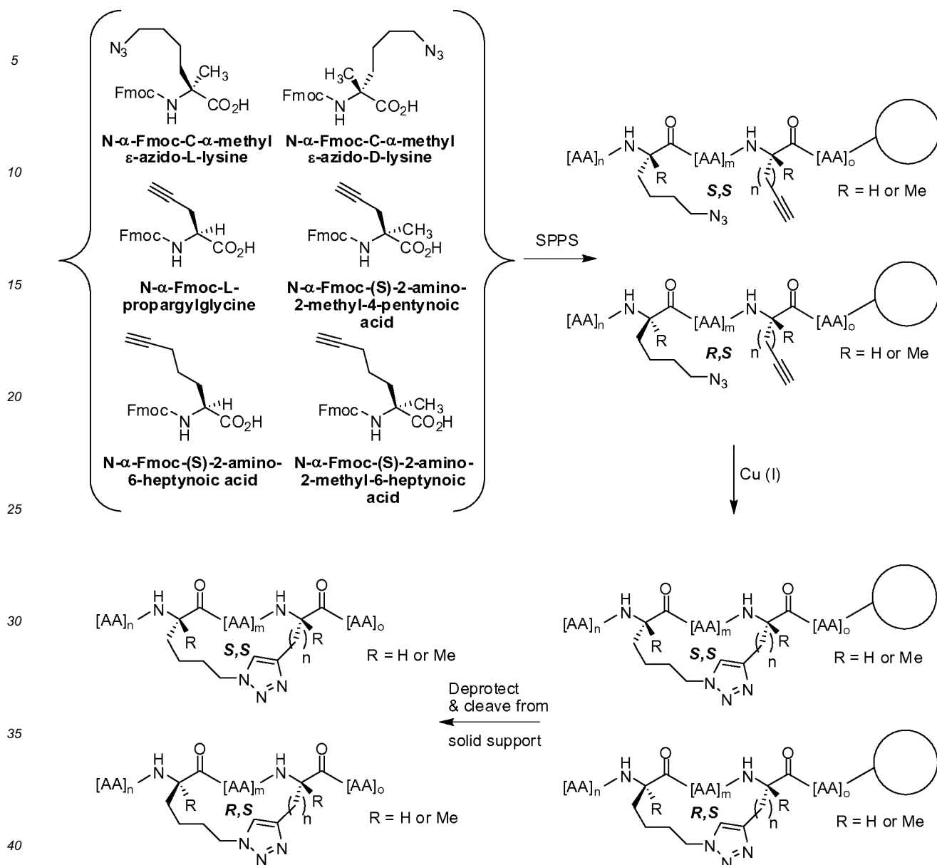
Synthetic Scheme 3:
