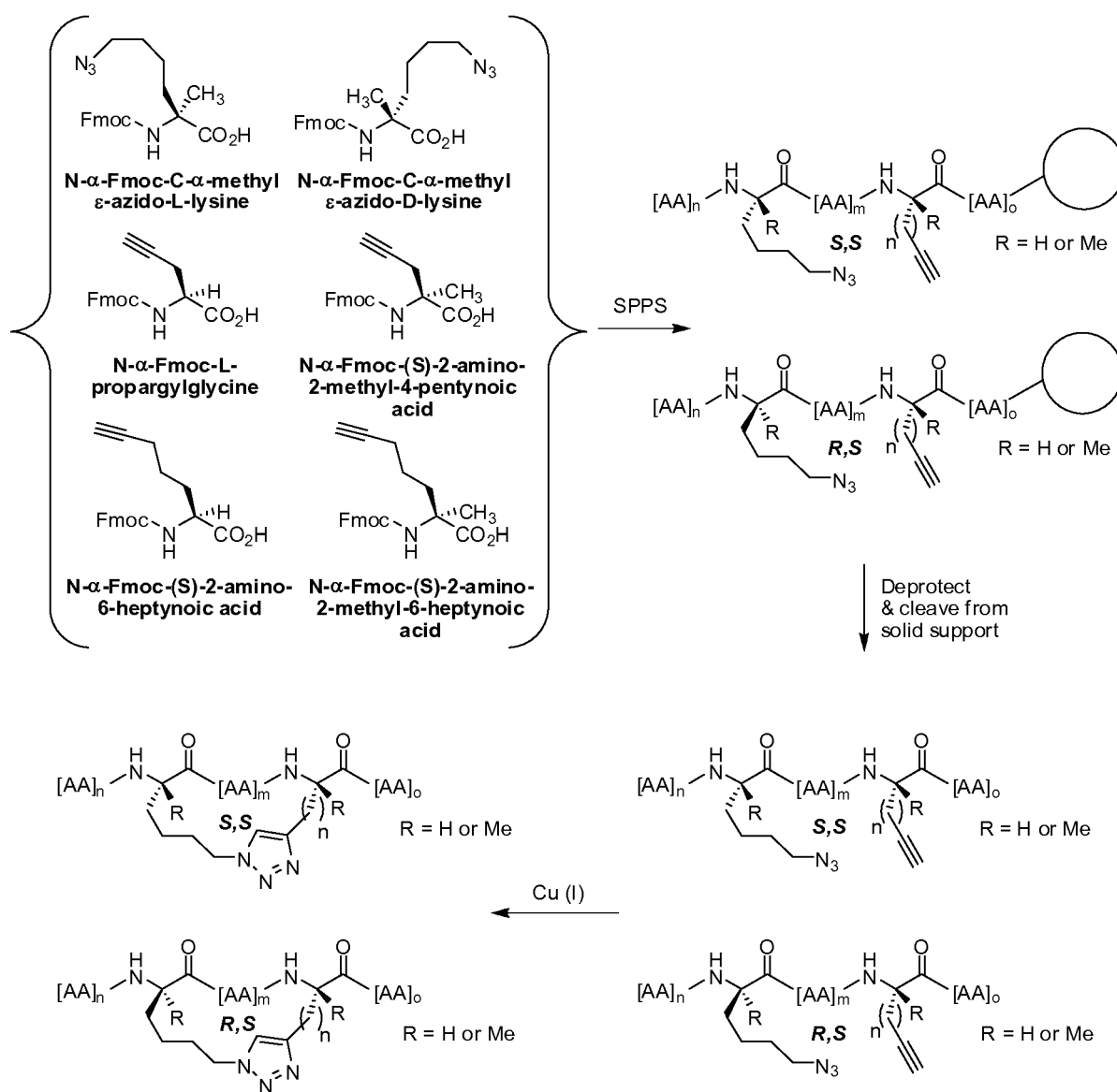
Synthetic Scheme 2:
