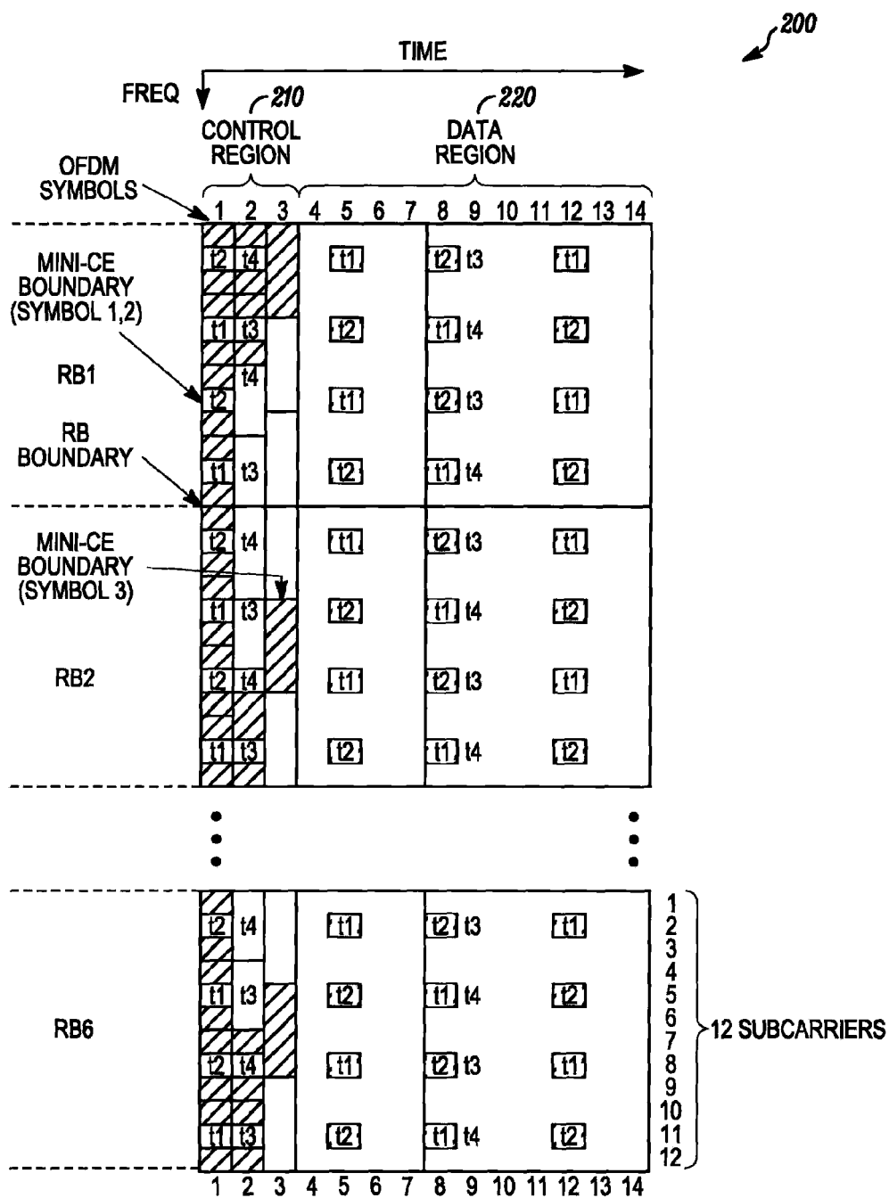
FDD DOWNLINK SUB-FRAME FOR 1.25 MHz CARRIER
