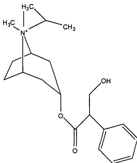
Ipratropium
