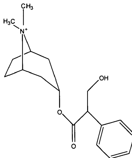
Methyl-atropine
