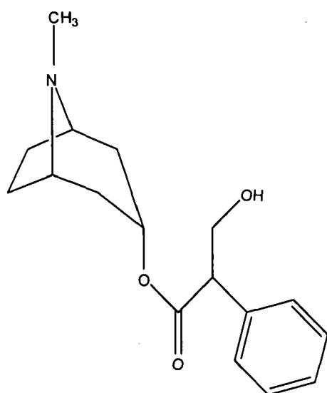
Atropine
