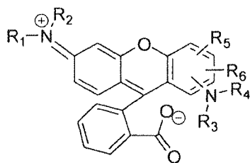
Structure I
