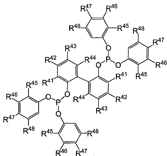
Formula X
