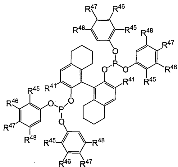
Formula XI
