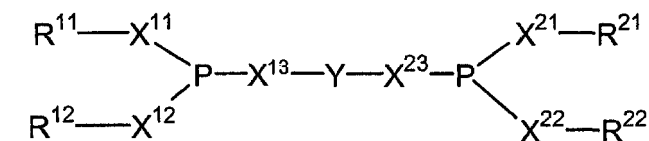
Formula III
