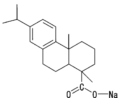
Compound No. 6
