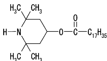
Compound No. 20
