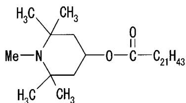
Compound No. 20
