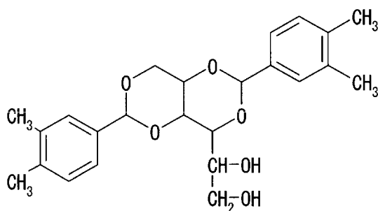
Compound No. 14
