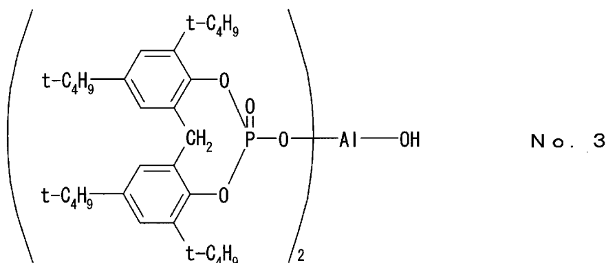
Compound No. 3
