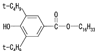
Compound No. 22
