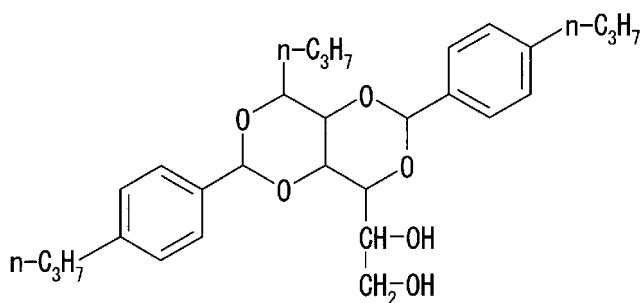
Compound No. 15
