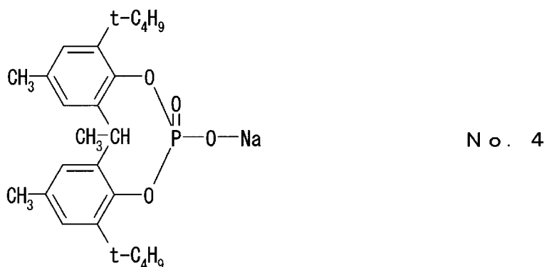
Compound No. 4
