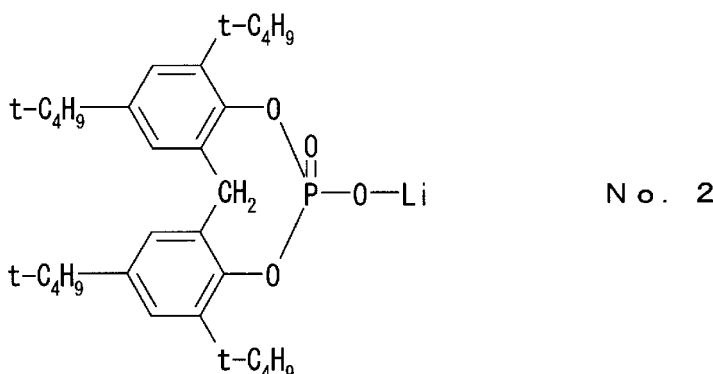
Compound No. 2
