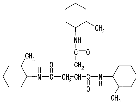
Compound No. 18
