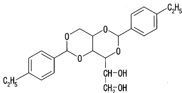
Compound No. 15
