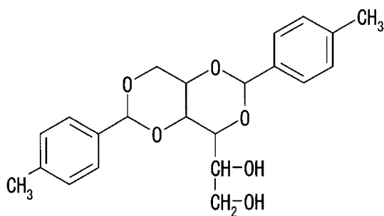
Compound No. 13
