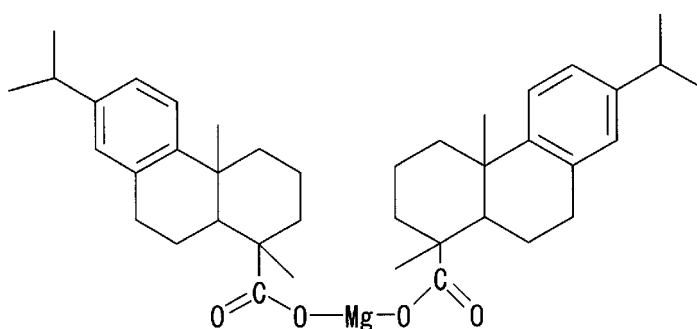
Compound No. 7
