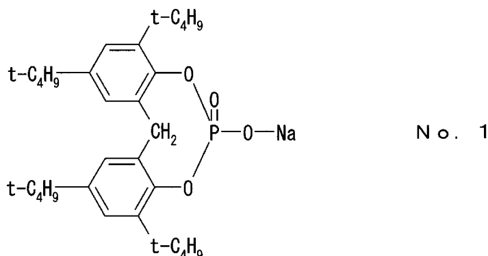
Compound No. 1
