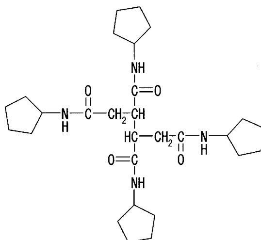
Compound No. 18
