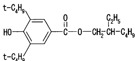
Compound No. 22
