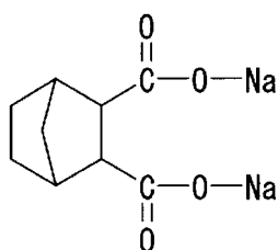
Compound No. 5
