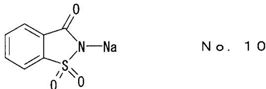
Compound No. 10
