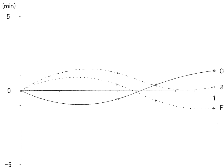
LATERAL CHROMATIC ABERRATION
