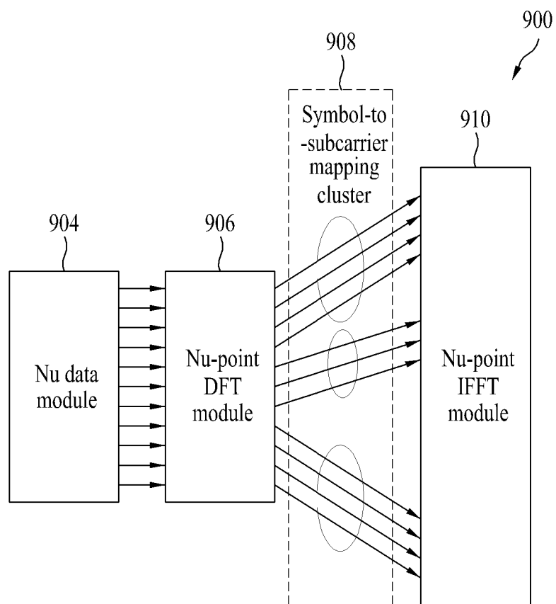
Clusters DFT-s-OFDMA
