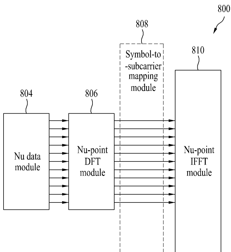
Localized DFT-s-OFDMA
