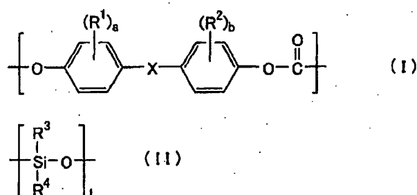
[Chem. 2]
