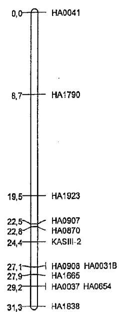
Figure 3: Co-localization of the low palmitic acid QTL (Panel A) and fatty acid gene KASIII-2 (Panel B) on LG 5.
