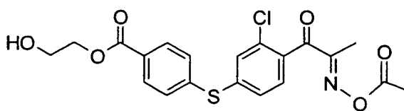
Compound No. 12
