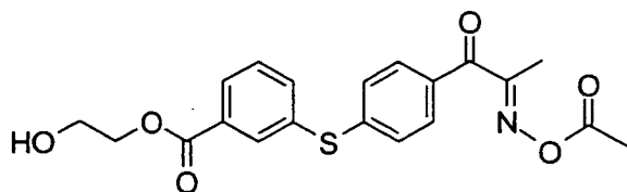
Compound No. 19
