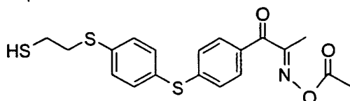
Compound No. 96
