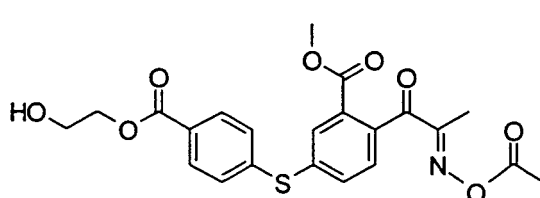
Compound No. 52
