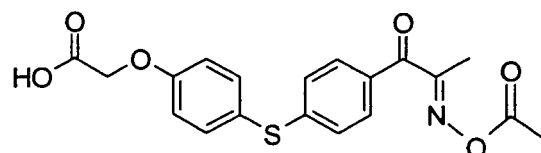
Compound No. 44
