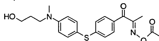
Compound No. 95
