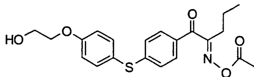
Compound No. 65
