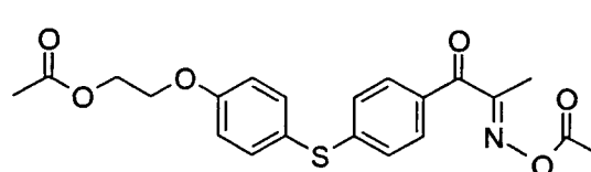
Compound No. 103
