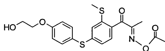
Compound No. 58
