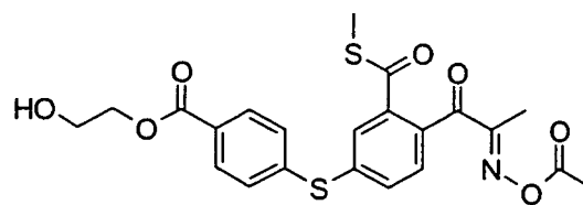
Compound No. 68
