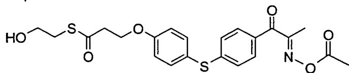
Compound No. 82
