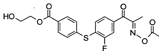
Compound No. 14
