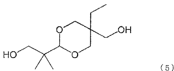
[Chem. 10]
