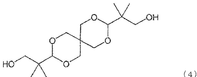
[Chem. 9]
