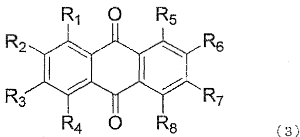
[Chem. 4]
