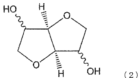
[Chem. 8]
