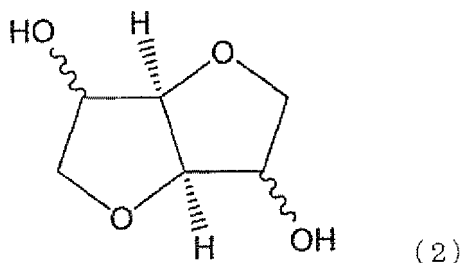
[Chem. 2]
