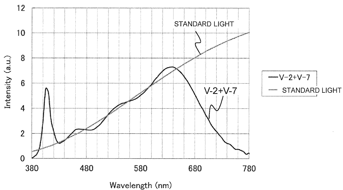
Fig.15 COMBINED SPECTRUM AND STANDARD LIGHT SPECTRUM
