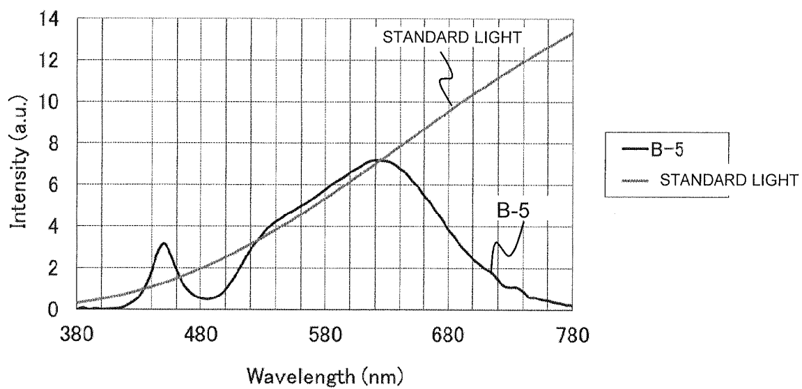
Fig.28 WHITE LED EMISSION SPECTRUM AND STANDARD LIGHT SPECTRUM
