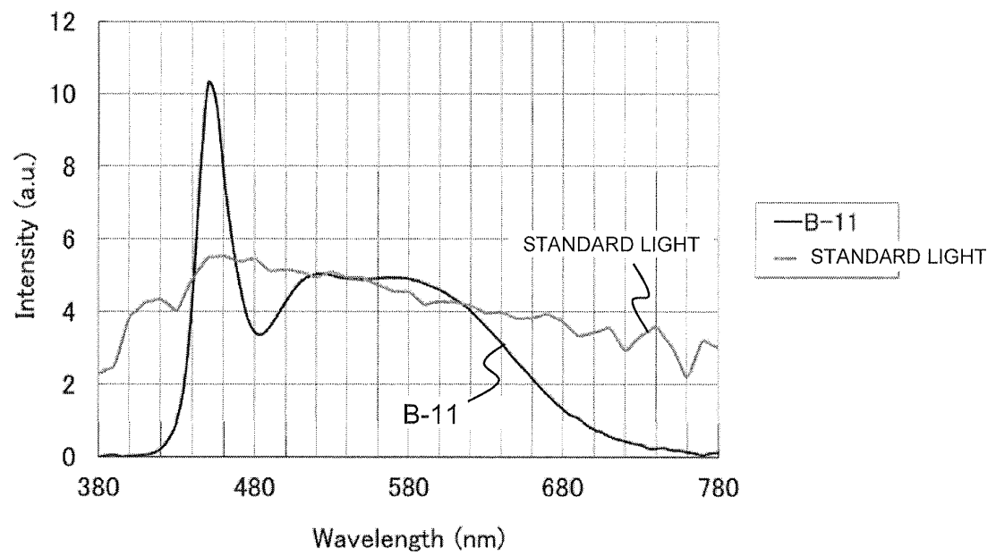
Fig.43 WHITE LED EMISSION SPECTRUM AND STANDARD LIGHT SPECTRUM
