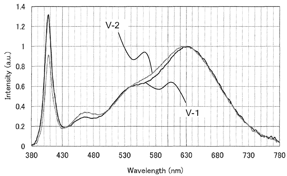
Fig.11 WHITE LED EMISSION SPECTRUM
