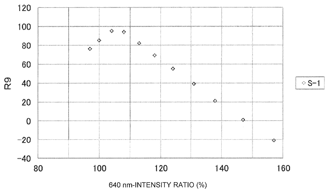
Fig.34 RELATIONSHIP BETWEEN 640 nm-INTENSITY RATIO AND R9
