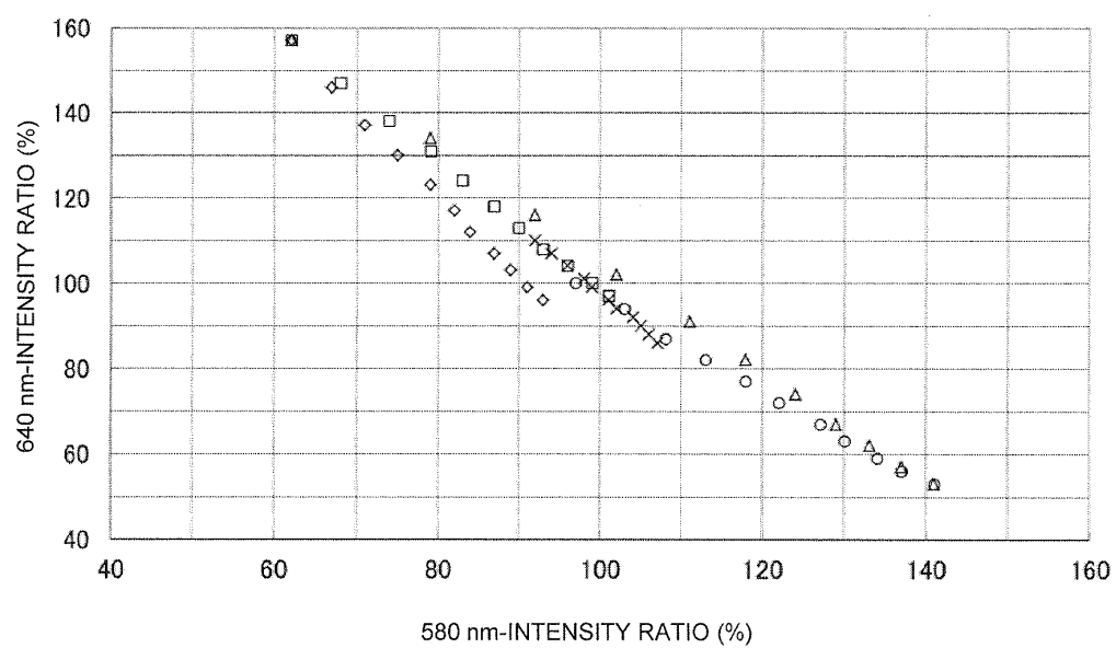
Fig.37 RELATIONSHIP BETWEEN 580 nm-INTENSITY RATIO AND 640 nm-INTENSITY RATIO
