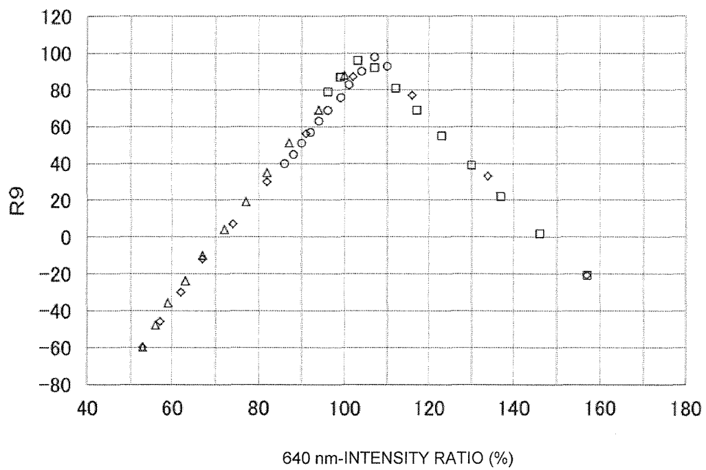
Fig.35 RELATIONSHIP BETWEEN 640 nm-INTENSITY RATIO AND R9
