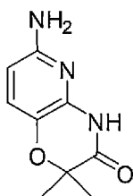
6-amino-2,2-dimethyl-2H-pyrido[3,2-b][1,4]oxazin-3(4H)-one
