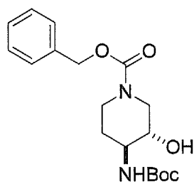
(trans)-Benzyl 4-((tert-butoxycarbonyl)amino)-3-hydroxypiperidin-1-carboxylate
