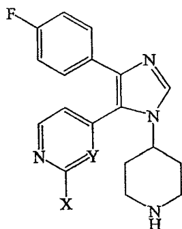
P6 X = H, Y = CH; HEP 689 (SB 235699)
