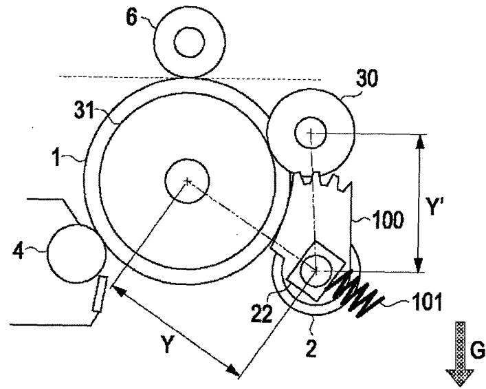
(a) SPACED
