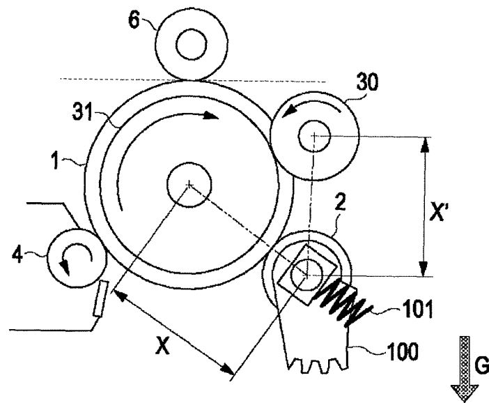
(b) CONTACTED
