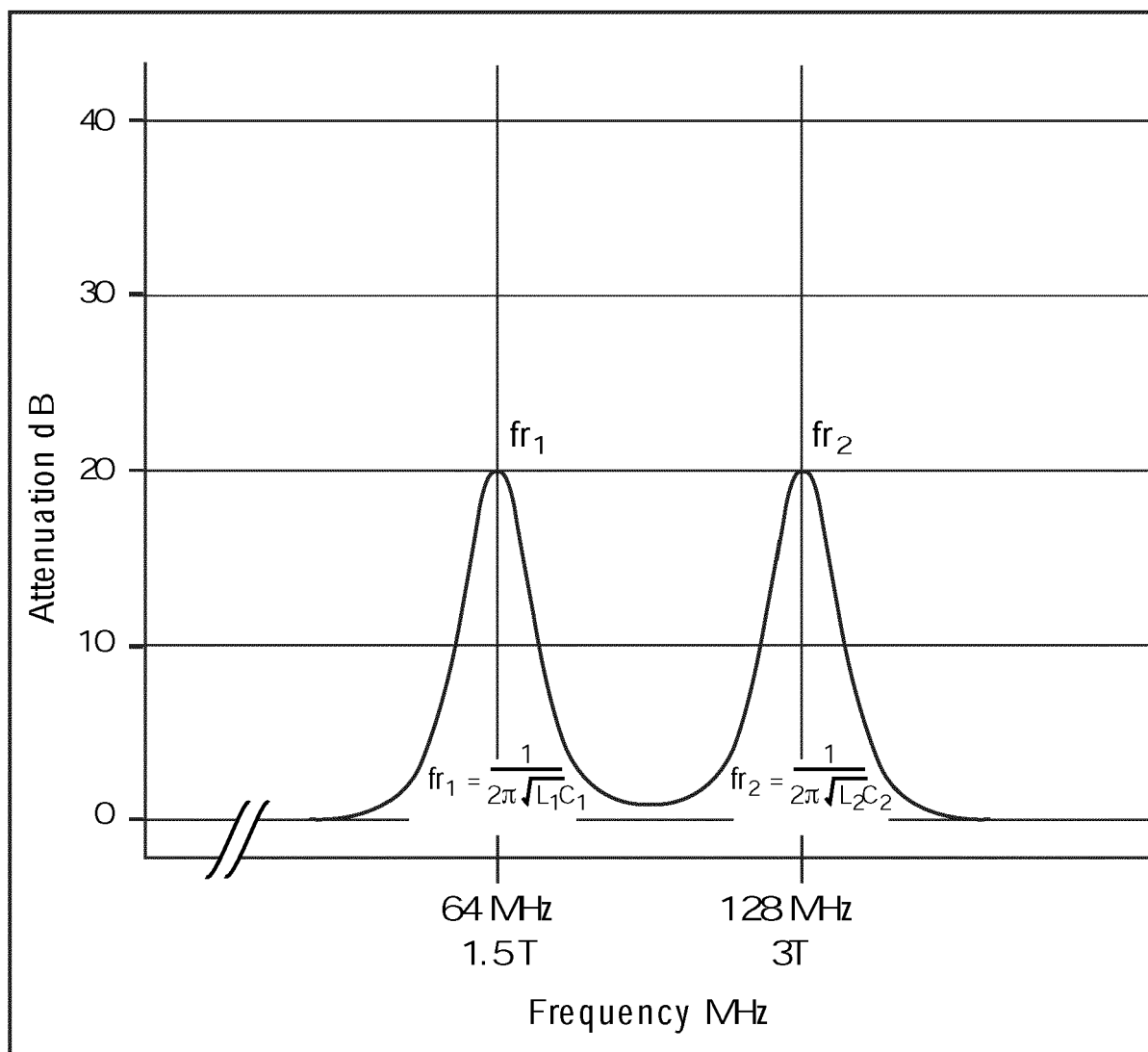
FIG. 24 PRIOR ART
