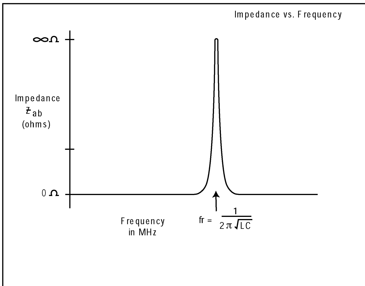
FIG. 18 PRIOR ART
