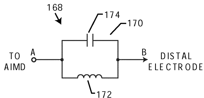
FIG. 16 PRIOR ART
