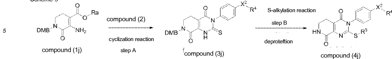
Scheme 9
