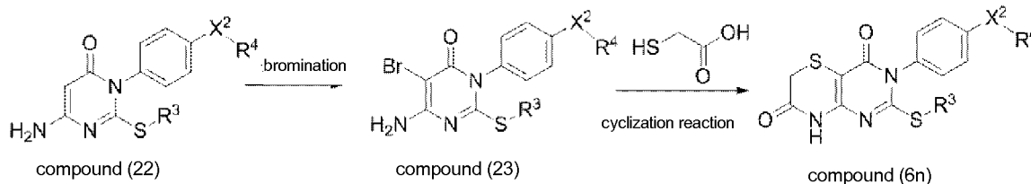
Scheme 15
