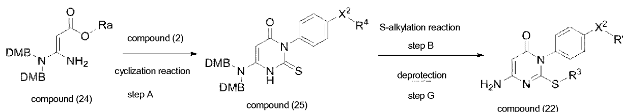
Scheme 16
