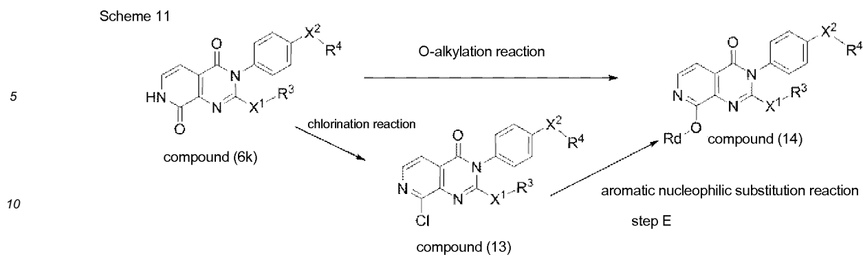
Scheme 11
