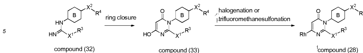
Scheme 20
