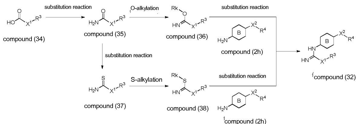
Scheme 21
