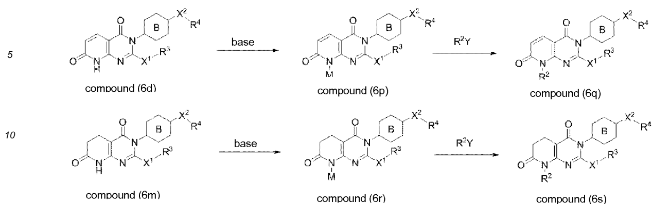
Scheme 18
