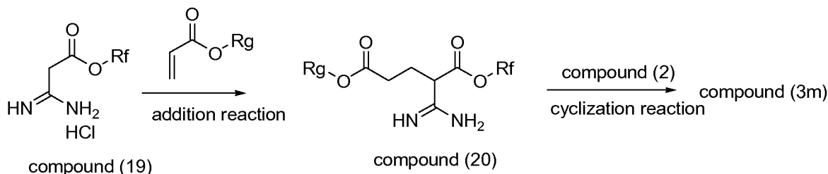
Scheme 14
