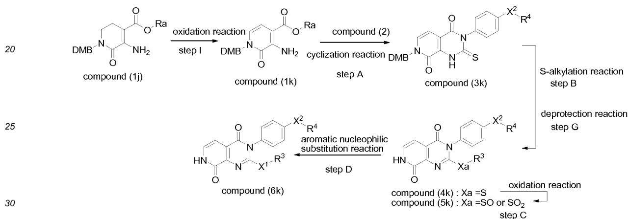
Scheme 10
