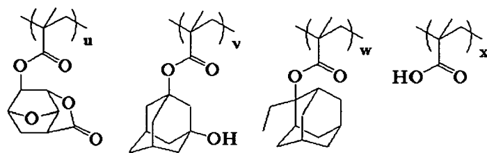
ArF single layer resist polymer 1 ( u=0.45, v=0.20, w=0.30, x=0.05 Mw7,800)
