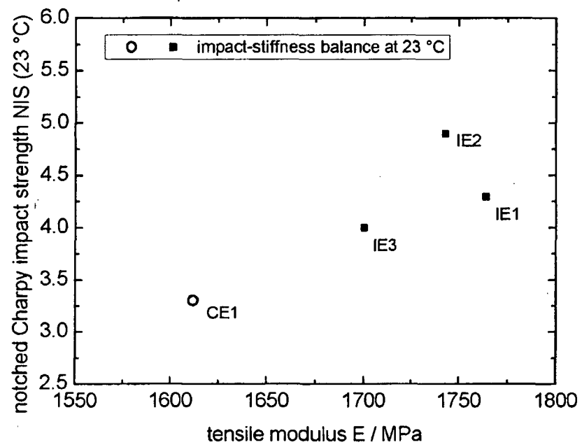
- Figure 1: Impact stiffness balance at 23 °C
