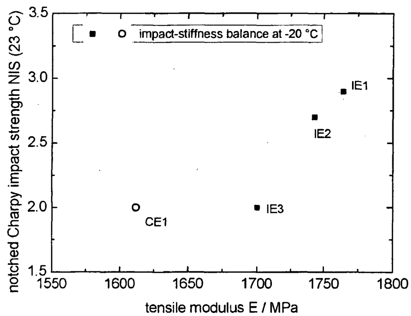
- Figure 2: Impact stiffness balance at -20 °C
