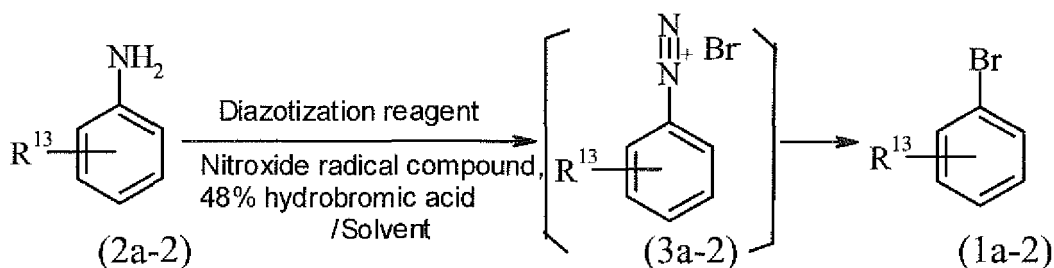
[Scheme 2a]
