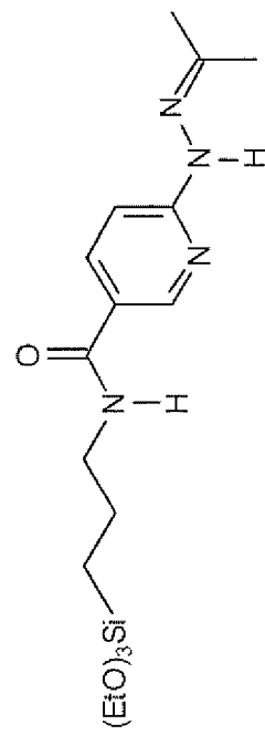
HyNic silane
