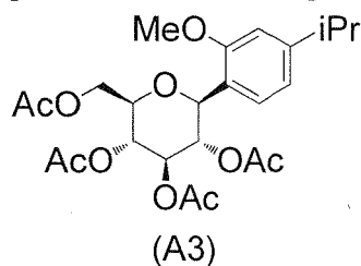
[Chemical Formula 9]
