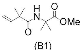
[Chemical Formula 16]
