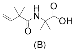
[Chemical Formula 15]
