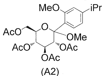
[Chemical Formula 8]
