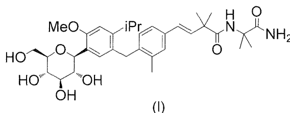
[Chemical Formula 24]
