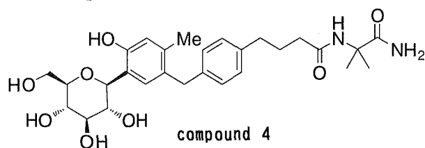
[Chemical Formula 25]
