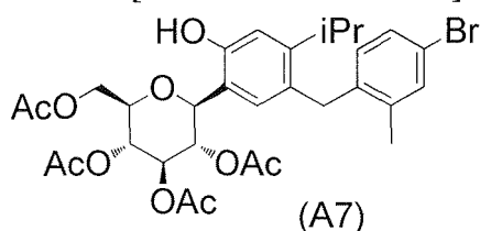
[Chemical Formula 14]
