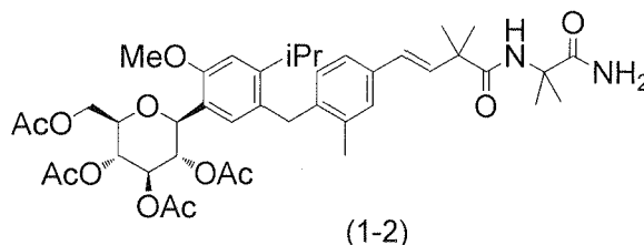
[Chemical Formula 23]
