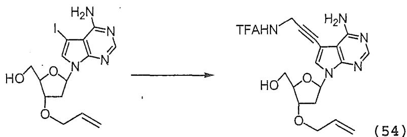
3'-O-Allyl-7-deaza-7-[3-(2,2,2-trifluoroacetamide)]-2'-deoxyadenosine (54).
