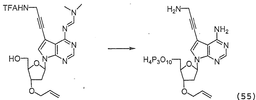
3'-O-Allyl-7-[3-aminoprop-1-ynyl]-7-deaza-2'-deoxyadenosine 5'-O-nucleoside triphosphate (55).
