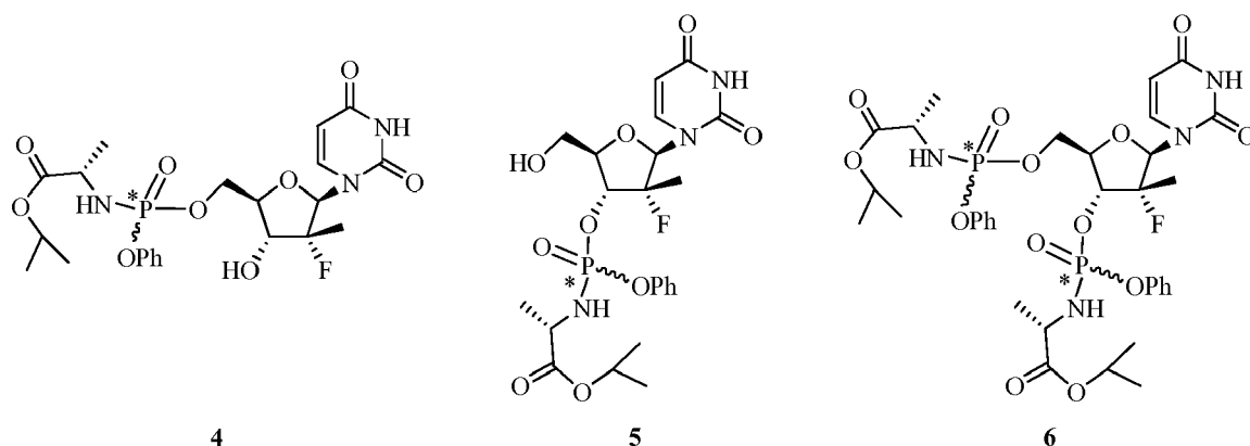
5'-O-phosphoramidate (2 diastereomers)
