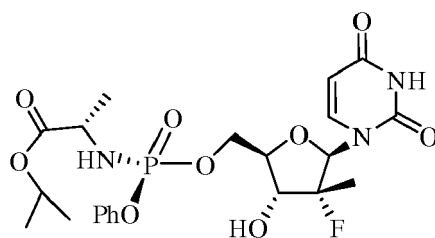
S_{P-4}
